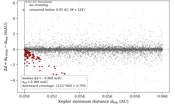
Fig. 4. Threshold censoring, measured directly. For the 17 469 pairs with Kepler distance in [0.05, 0.06) \text{ AU} — the band a 0.05 AU catalogue discards — re-refined under full N-body, \Delta d = d_{\text{N-body}} - d_{\text{Kep}} is plotted against d_{\text{Kep}} . The distribution is symmetric about zero (median 0.000 \text{ mAU} , \sigma = 0.366 \text{ mAU} ); the 122 pairs (0.70 %) that cross downward below 0.05 \text{ AU} (red) are the measured false-negatives, concentrated just above the threshold as expected for a scatter-dominated selection effect.
