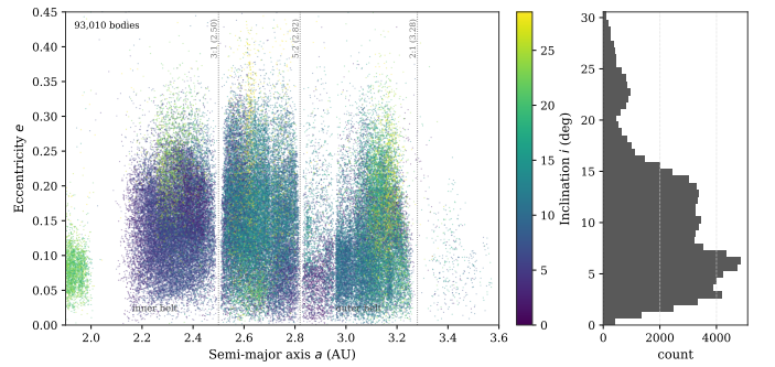
Fig. 3. Semimajor axis vs eccentricity of the 93 010 encountering bodies, coloured by inclination, with the inclination marginal at right. The 3:1, 5:2 and 2:1 mean-motion resonances (Kirkwood gaps) are marked.
