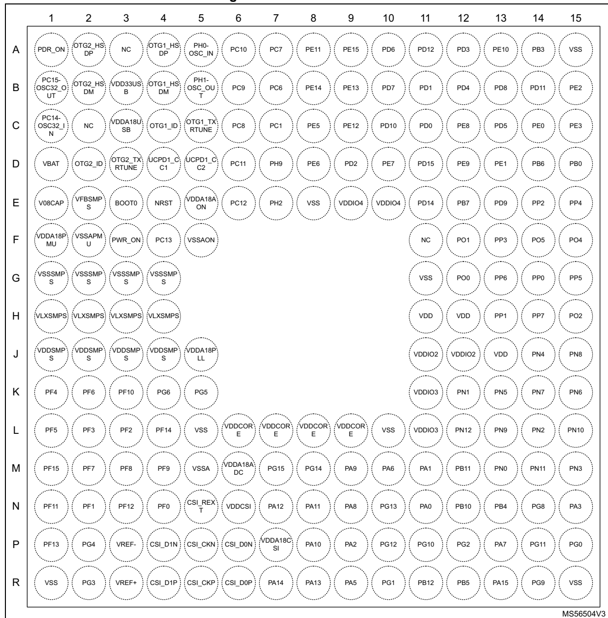
Figure 11. VFBGA198 ballout
