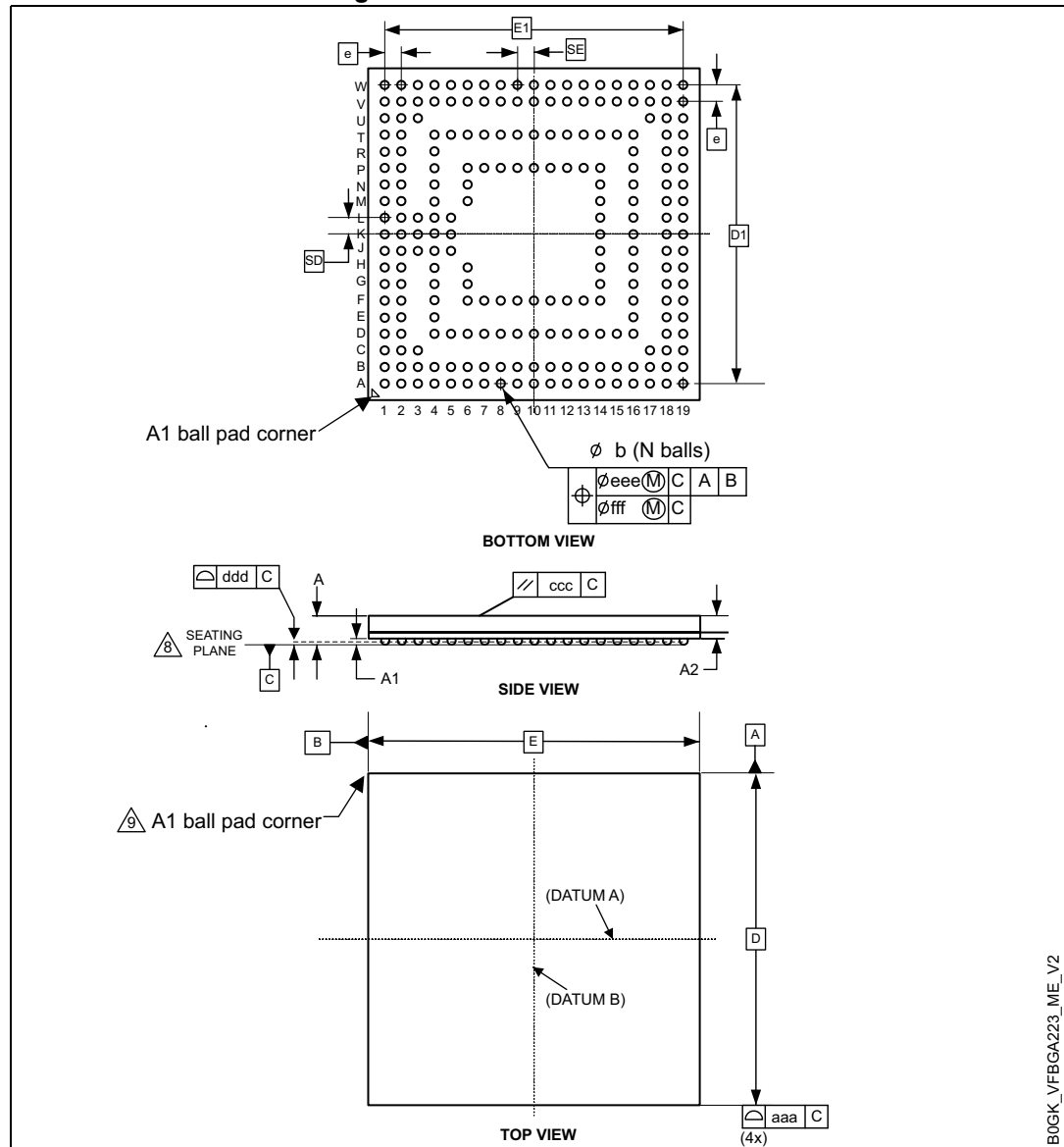
Figure 72. VFBGA223 - Outline (13)
