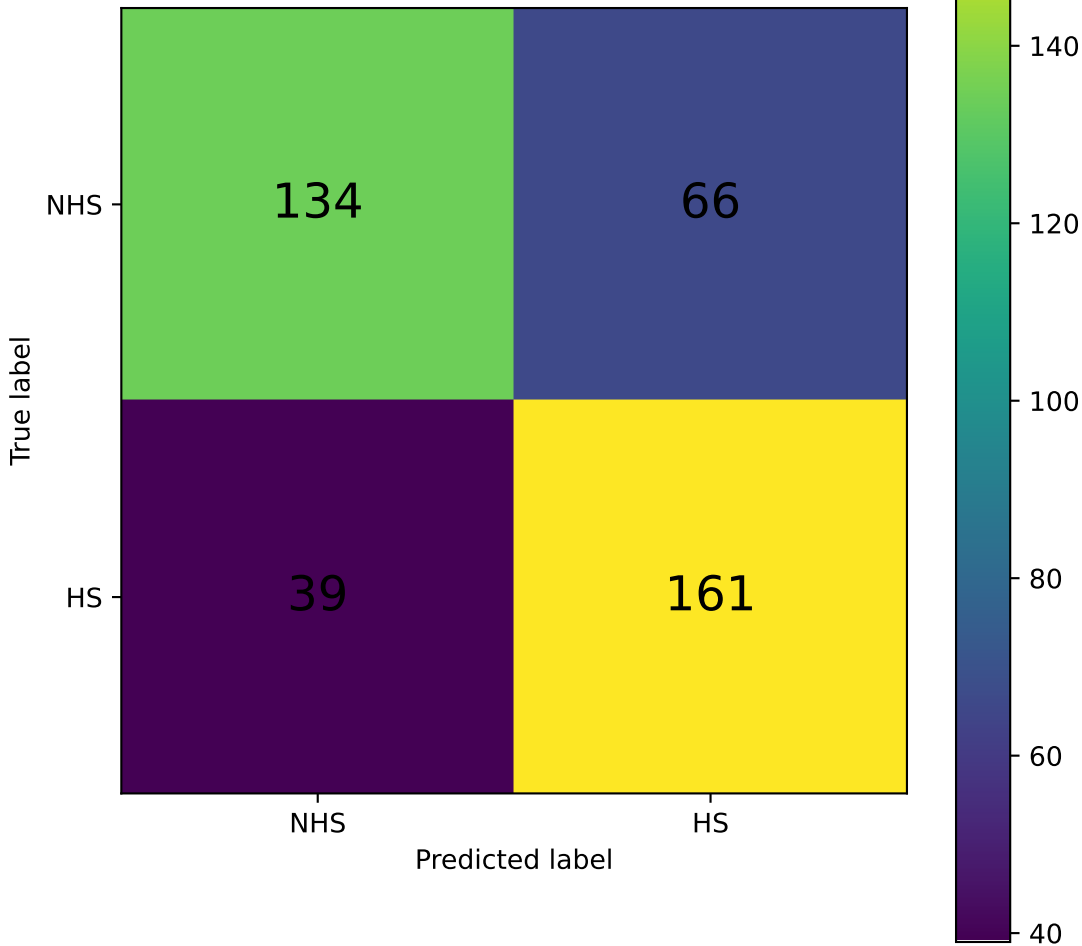
GPT-4.1-mini Overall Confusion Matrix
