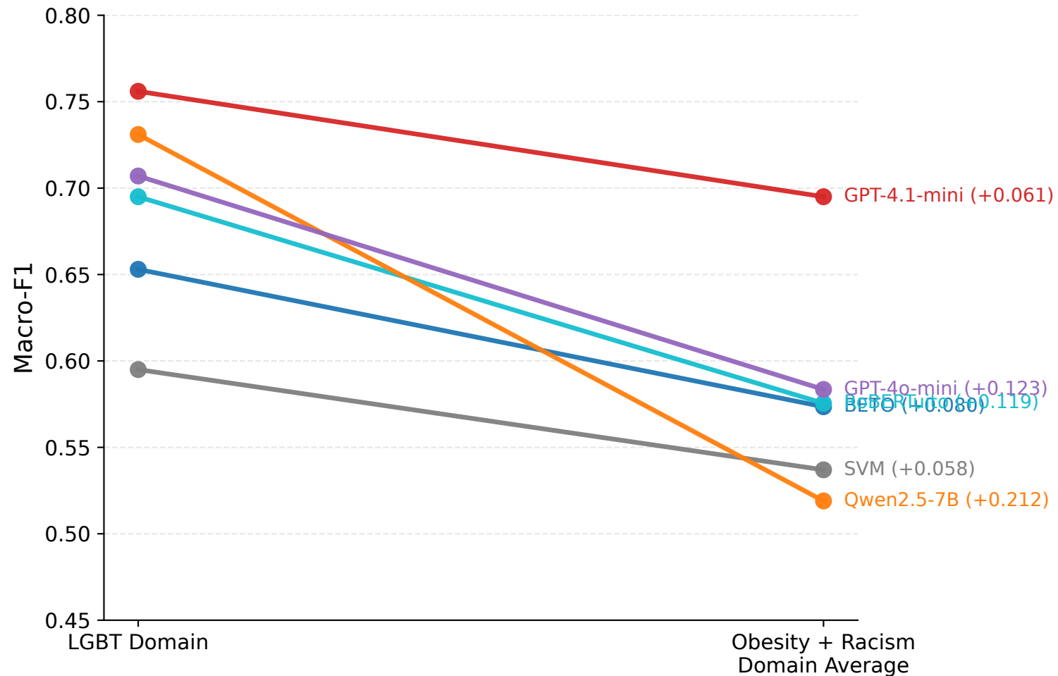
Cross-Domain Performance Variation Across Evaluated Models
