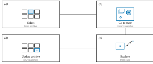
Figure 2. Search over Daytona sandboxes. (a) Select a snapshot from the archive. (b) Restore that sandbox (Go-Explore’s “go to state”). (c) A new agent explores from the restored machine. (d) New snapshots update the archive. Independent retry is the matched-budget baseline and is not shown.
