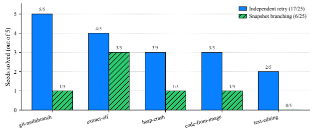
Figure 3. Pre-registered headline comparison. Five file-centric Terminal-Bench tasks \times five seeds, 1,000,000 tokens. Independent retry from scratch outperforms snapshot branching (17/25 versus 6/25). When useful progress is mostly in the filesystem, starting over is often enough. This total is frozen; later warehouse rows are not pooled into it.
