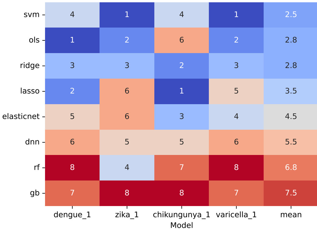
Rank of RMSE for each model and epidemic
