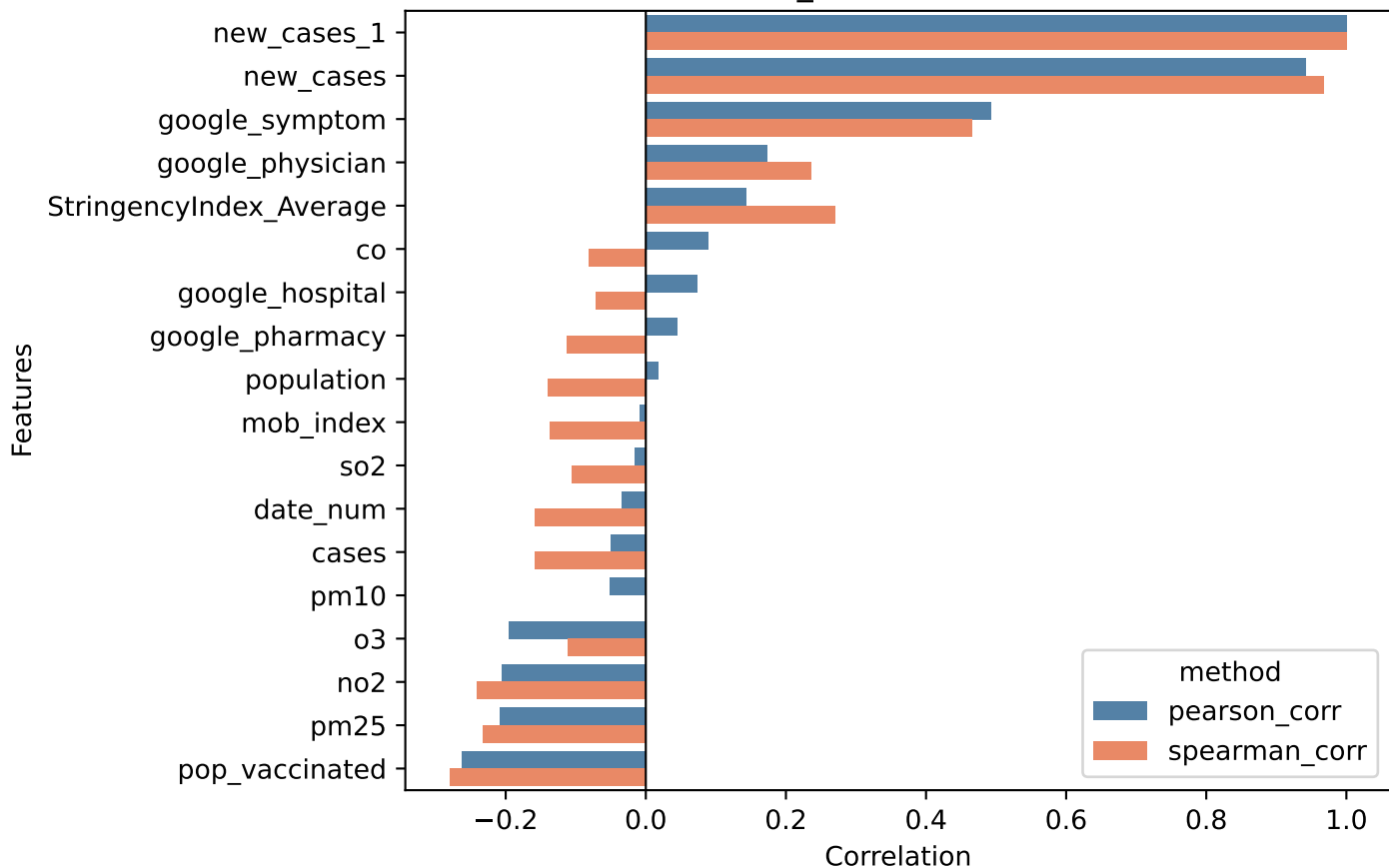
Correlation of new_cases at t+1 and features at t
