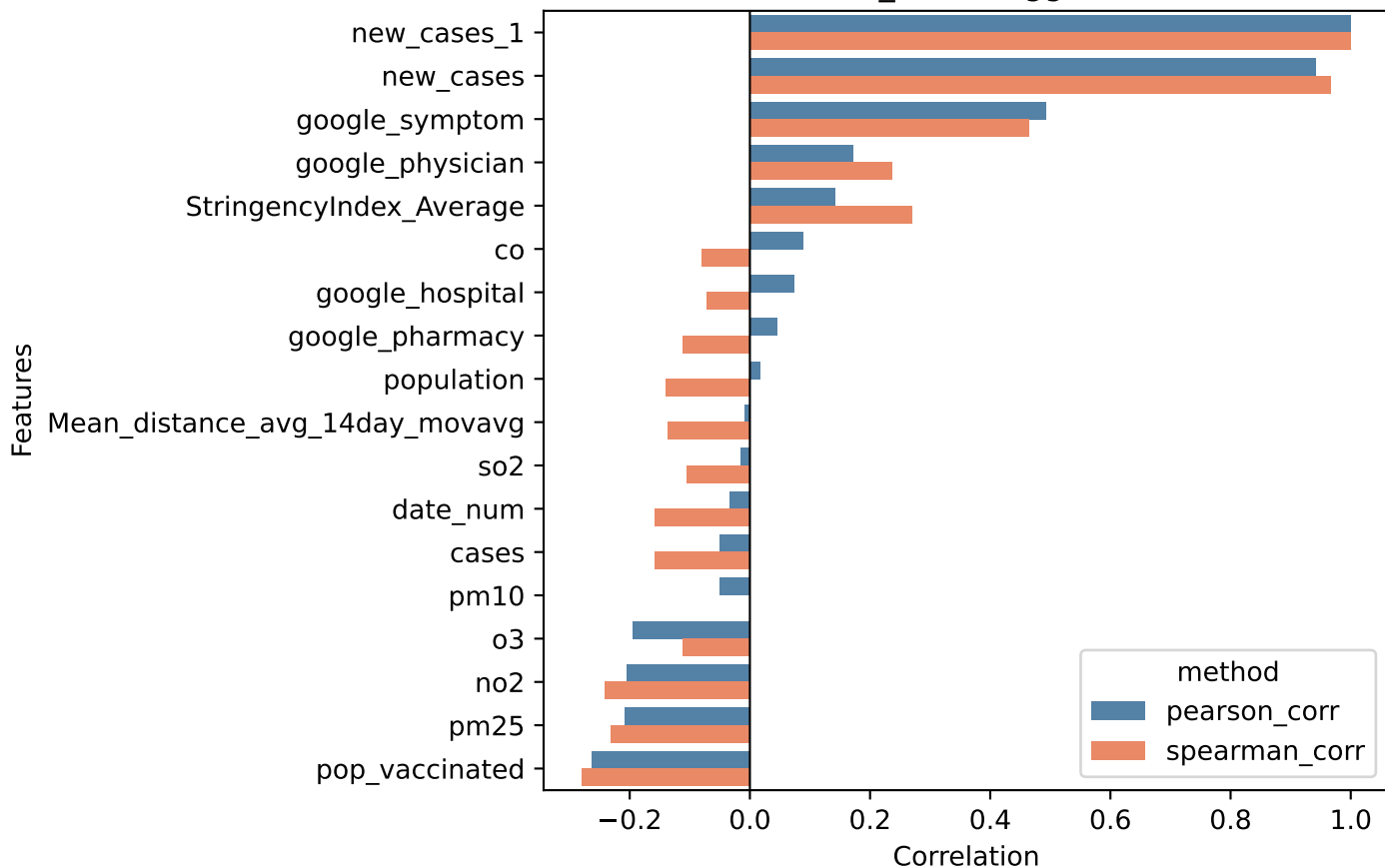
Correlation of new_cases lagged 1 and features
