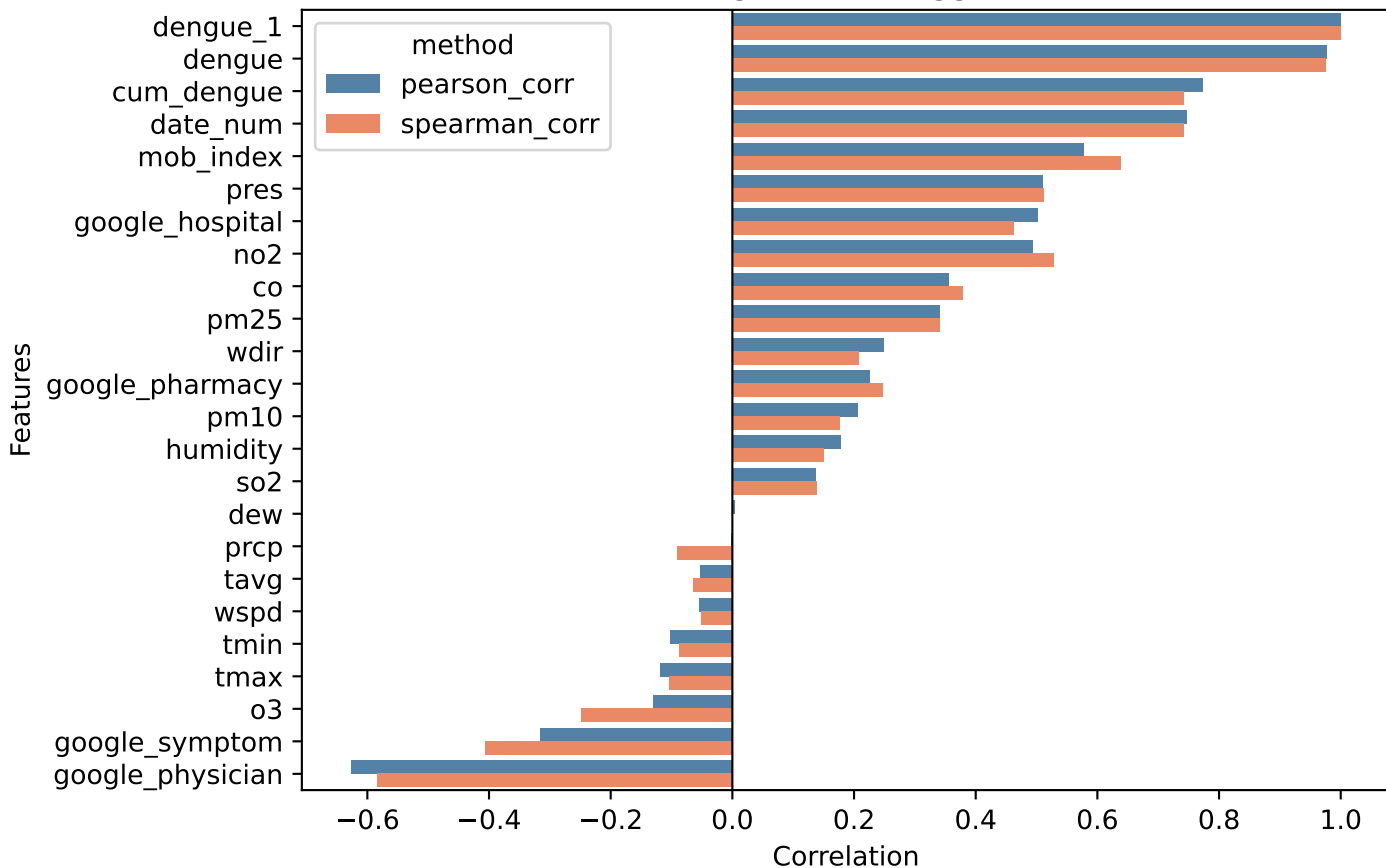
Correlation of Dengue cases lagged 1 and features
