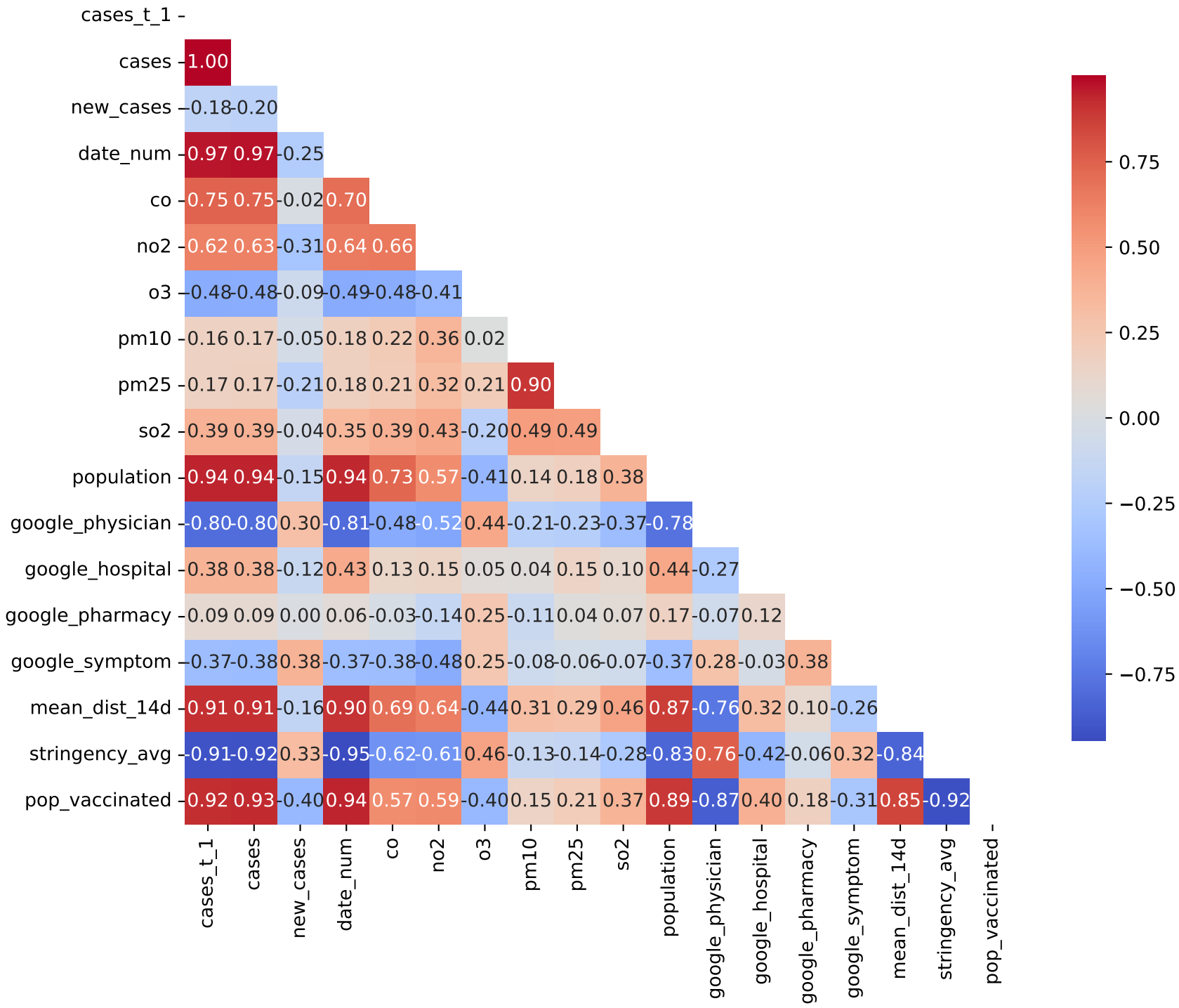
Lower Triangle Correlation Matrix for Colombia COVID-19 Data
