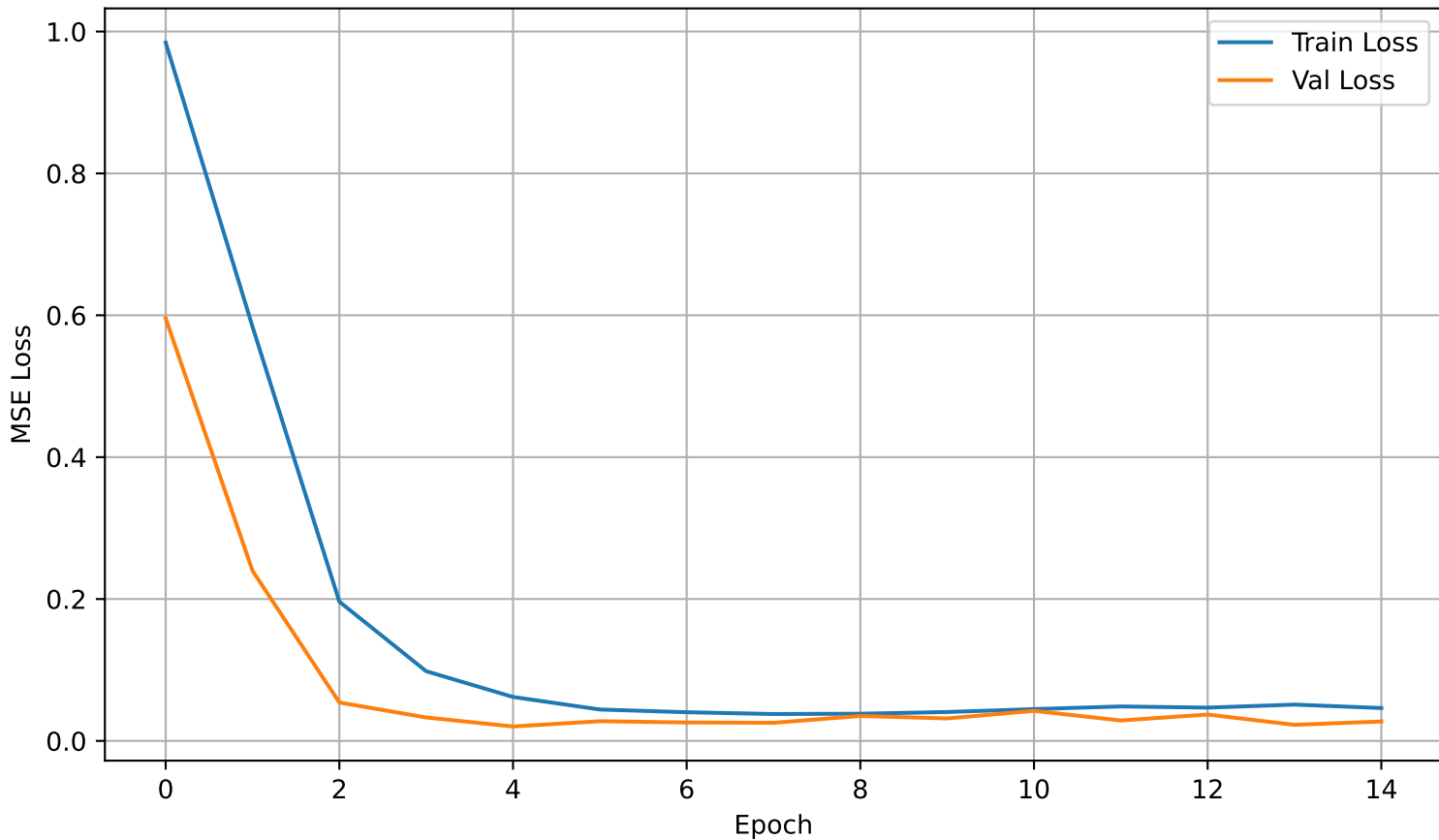
FFN Training & Validation Loss for Dengue
