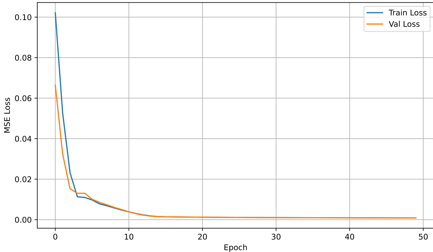
RNN Training & Validation Loss for Dengue
