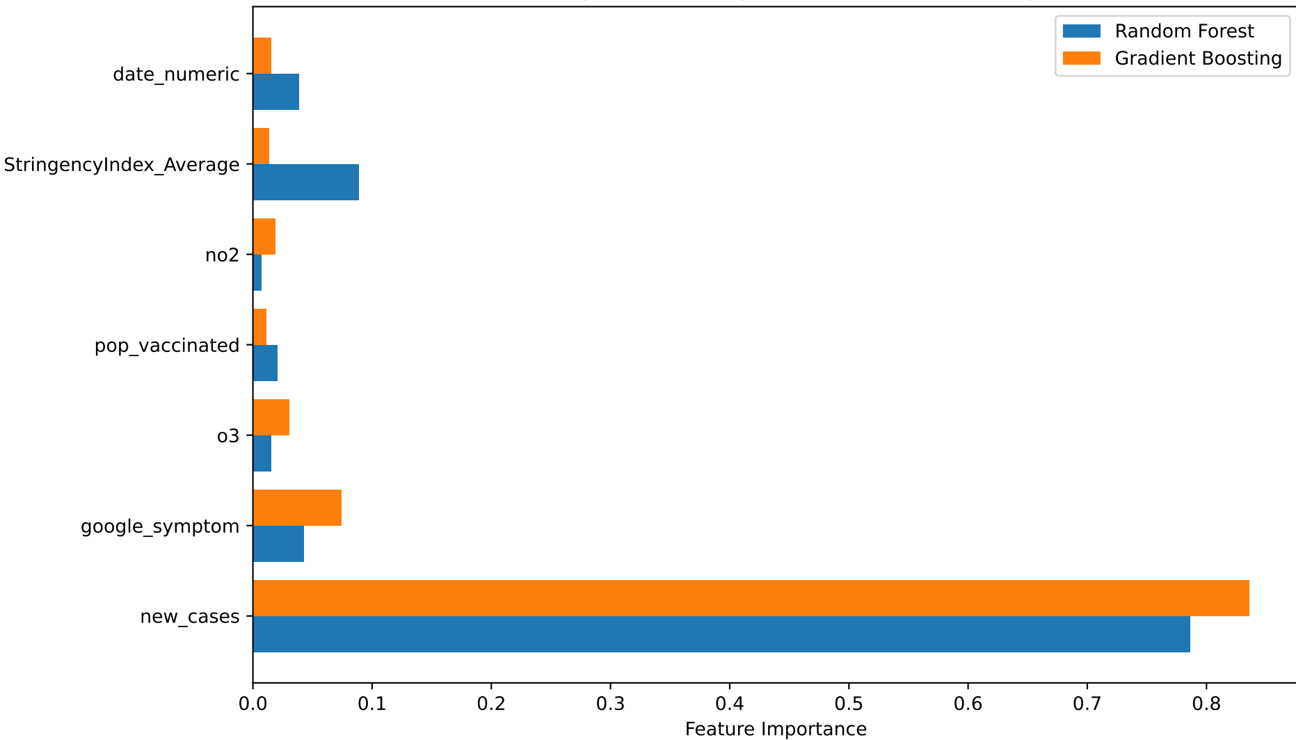
Feature Importance Comparison (Colombia Training Set)
