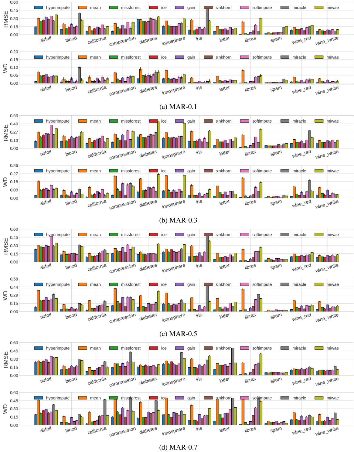
Figure 7: Overall Performance . Experiments on 12 UCI datasets under MAR simulations at four levels of missingness—{0.1, 0.3, 0.5, 0.7}. Results shown as mean \pm std of RMSE and WD.
