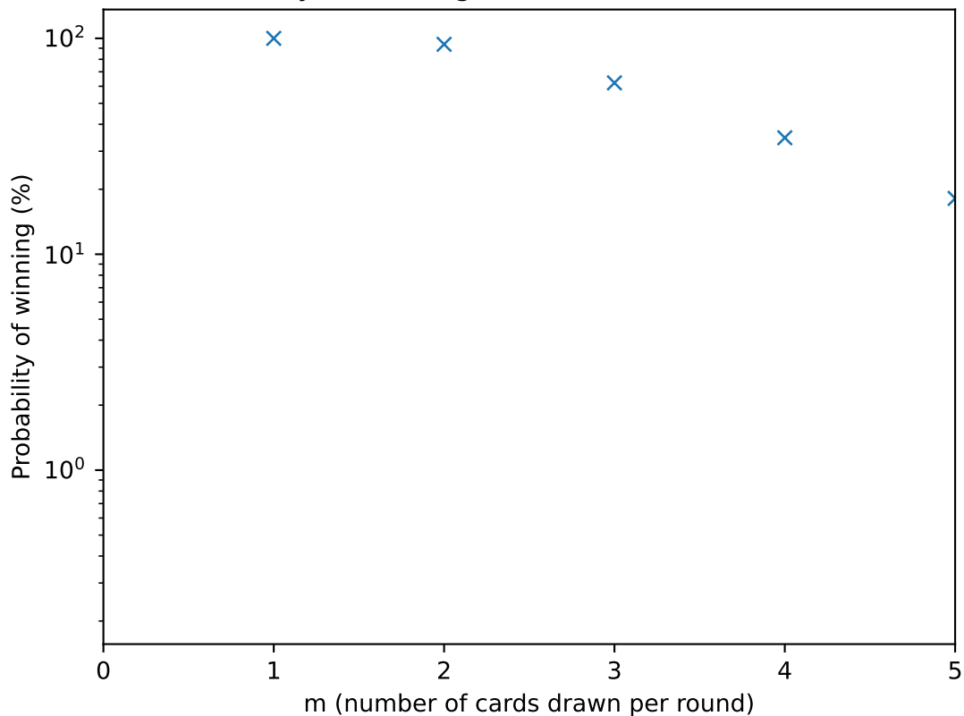
Probability of winning vs m (4 suits, 13 cards each)
