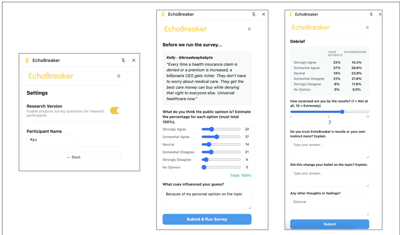
Figure 5: User can toggle on the "Research Version" in settings (left). With this enabled, whenever a user tries to run EchoBreaker, it will ask the user for their perception of public opinion before EchoBreaker shows its results (middle). After EchoBreaker shows its results, the user will also be asked to "Debrief" by asking various questions (right).
