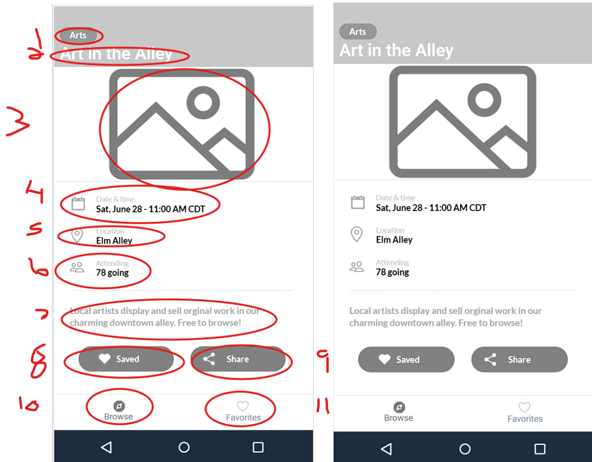
Figure 5 - Event Detail Screen
