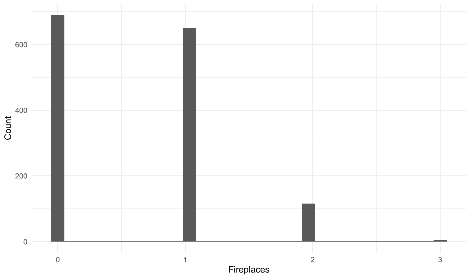
Histogram: Fireplaces
