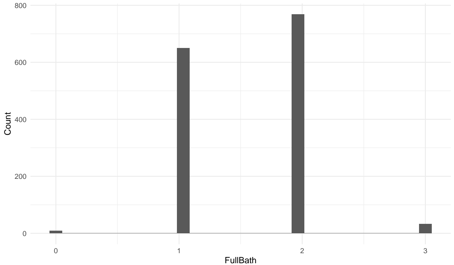
Histogram: FullBath
