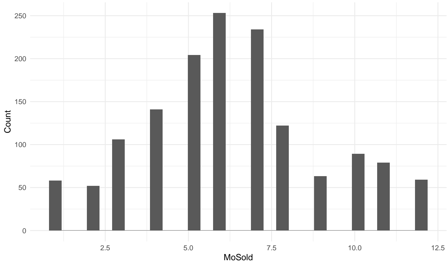
Histogram: MoSold
