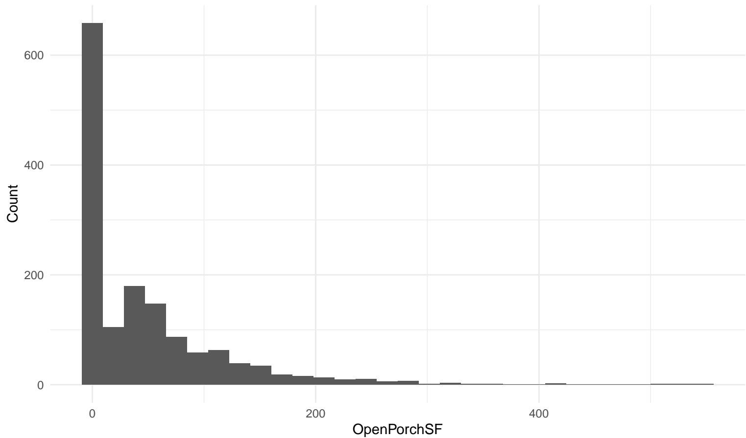
Histogram: OpenPorchSF
