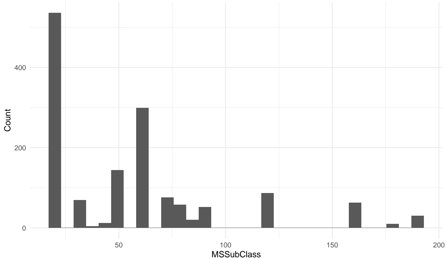
Histogram: MSSubClass
