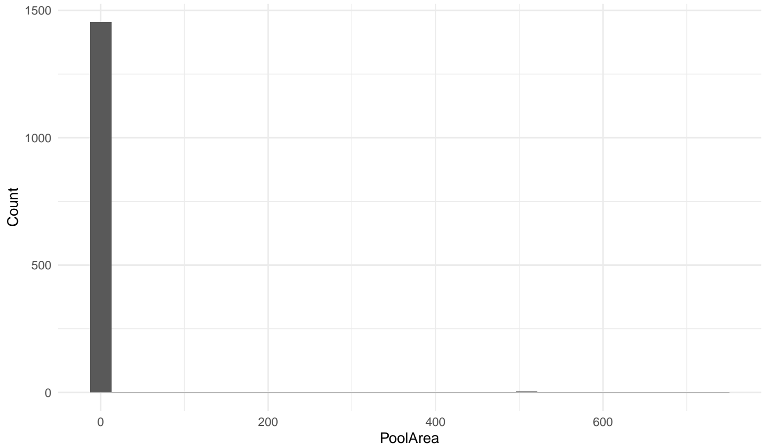
Histogram: PoolArea
