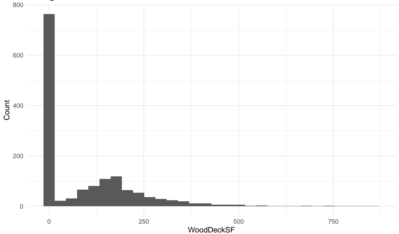
Histogram: WoodDeckSF
