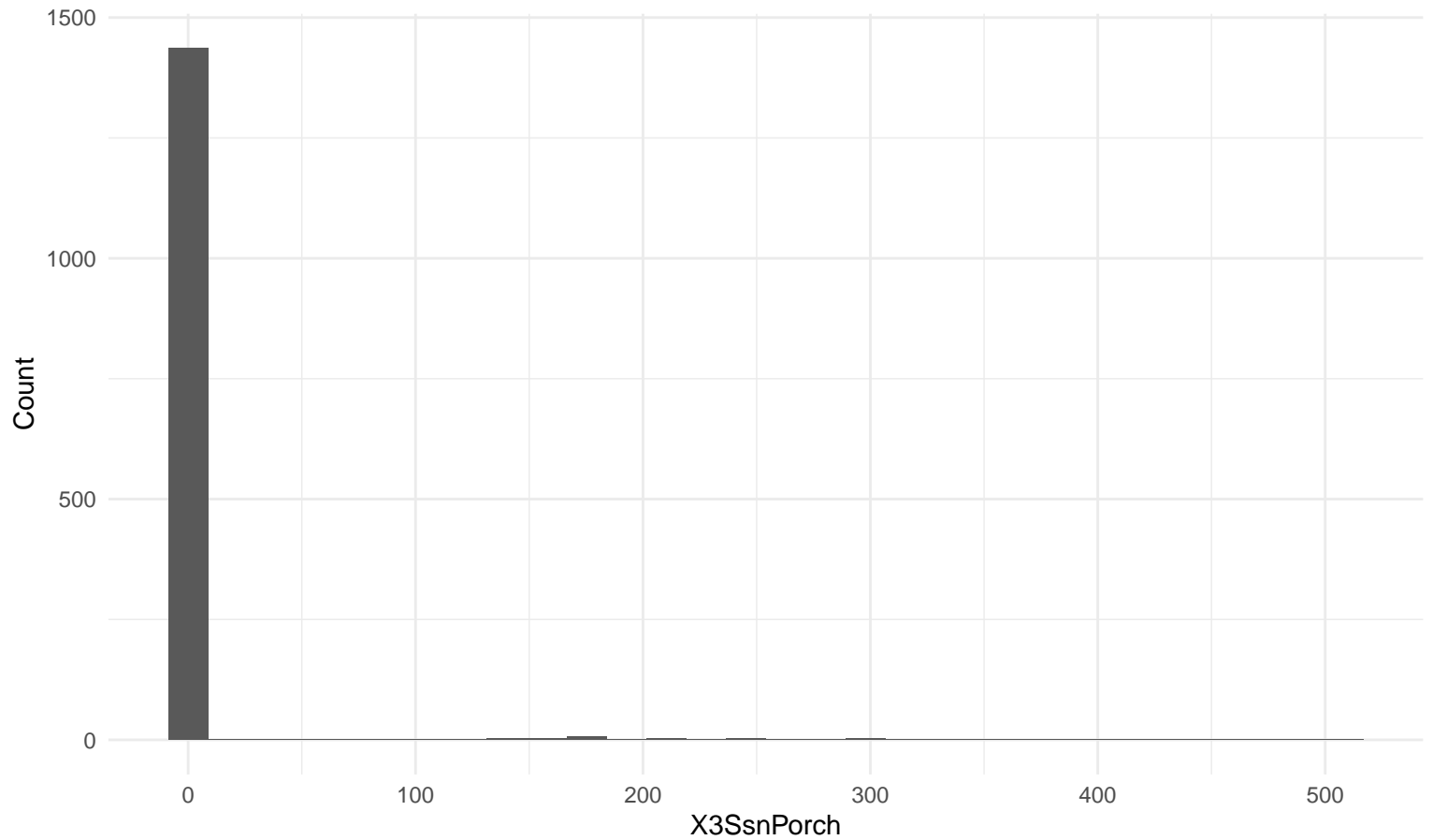
Histogram: X3SsnPorch
