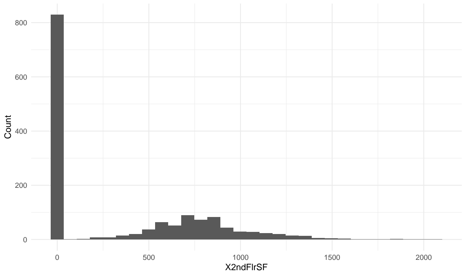
Histogram: X2ndFlrSF
