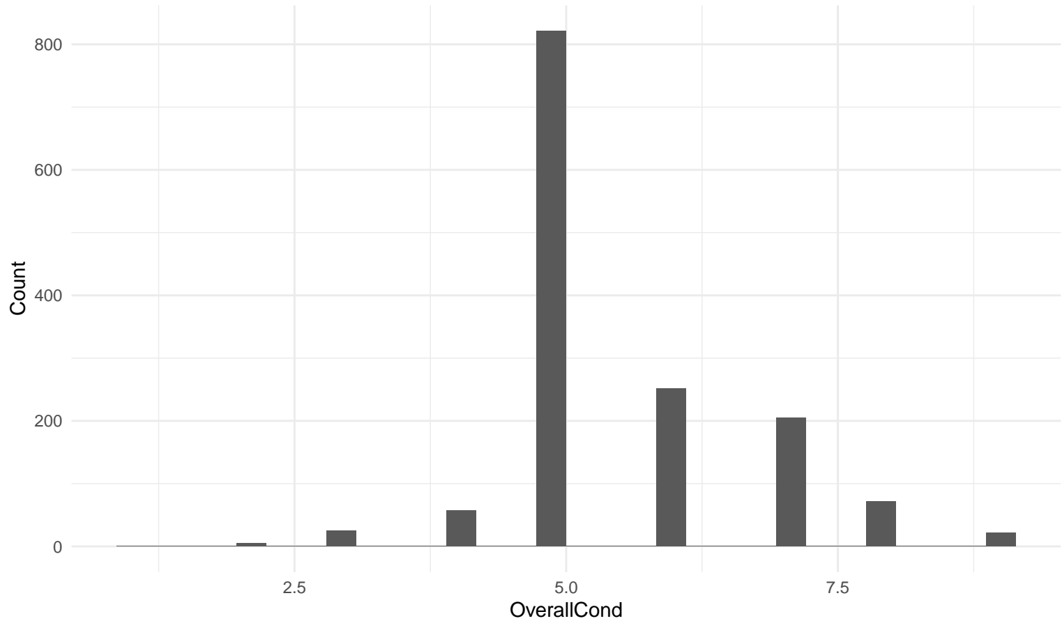
Histogram: OverallCond
