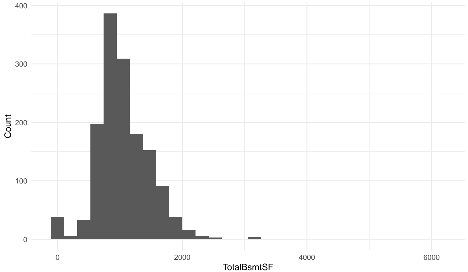
Histogram: TotalBsmtSF
