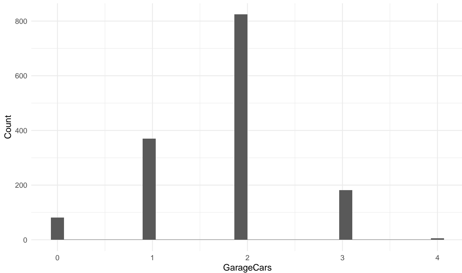
Histogram: GarageCars
