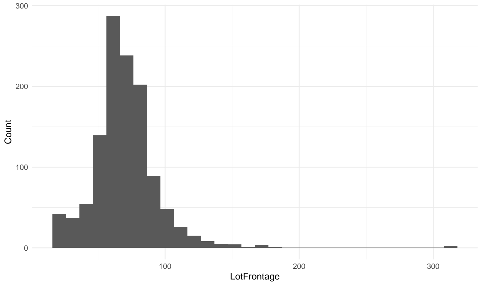
Histogram: LotFrontage
