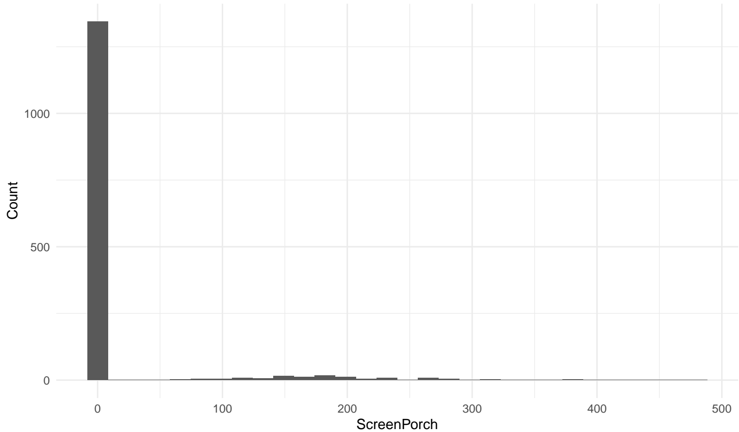
Histogram: ScreenPorch
