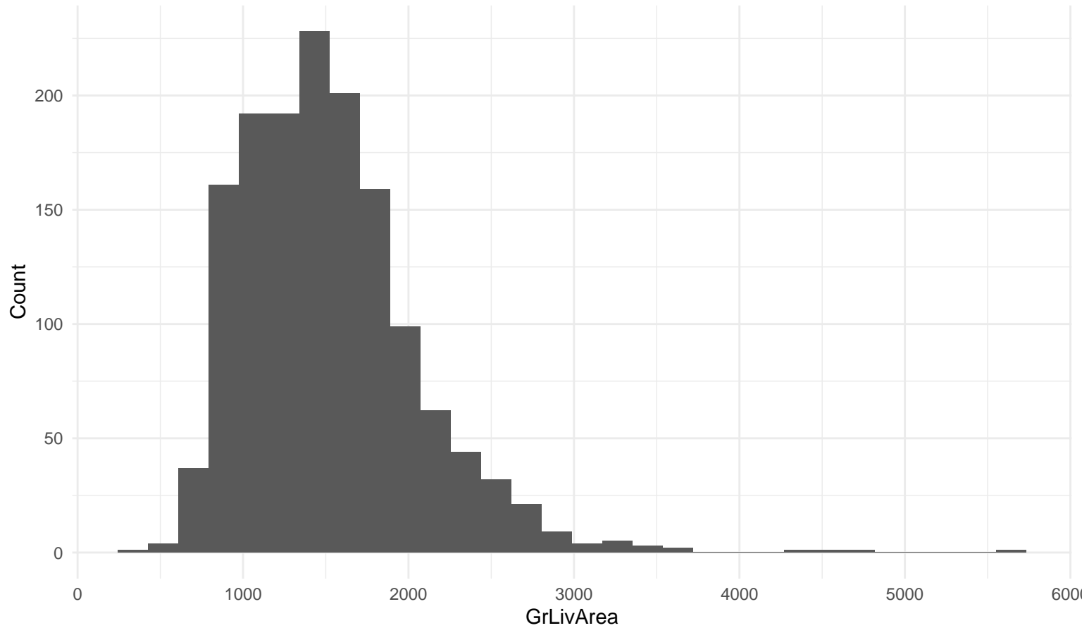
Histogram: GrLivArea
