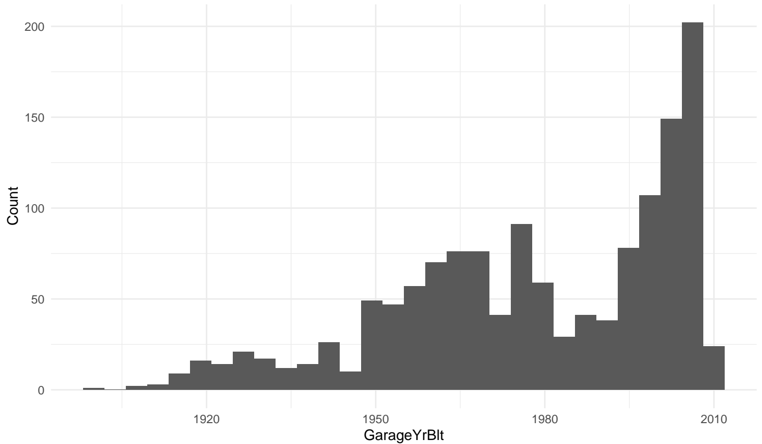
Histogram: GarageYrBlt
