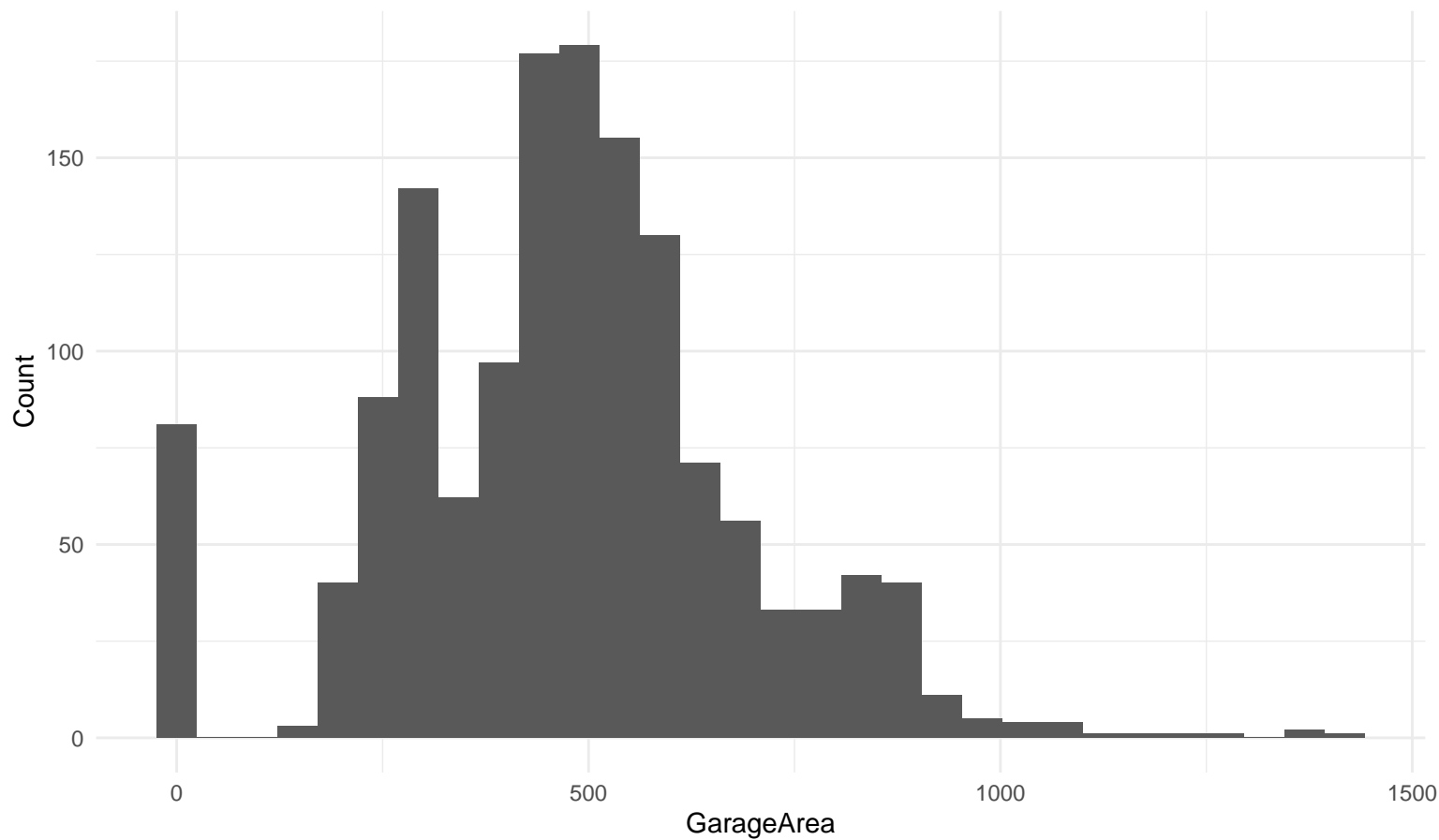
Histogram: GarageArea
