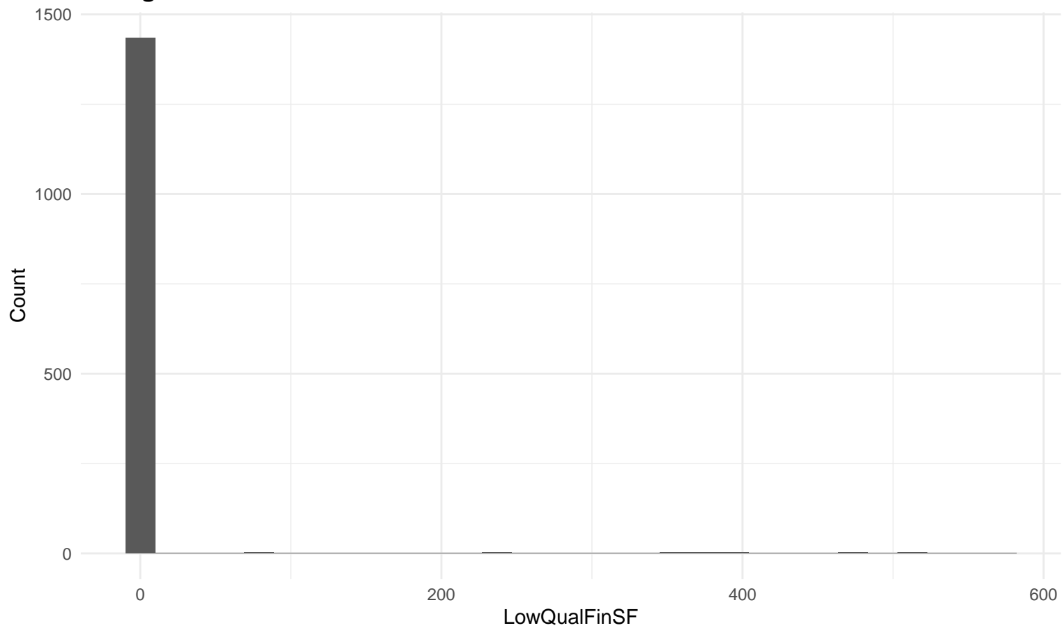
Histogram: LowQualFinSF
