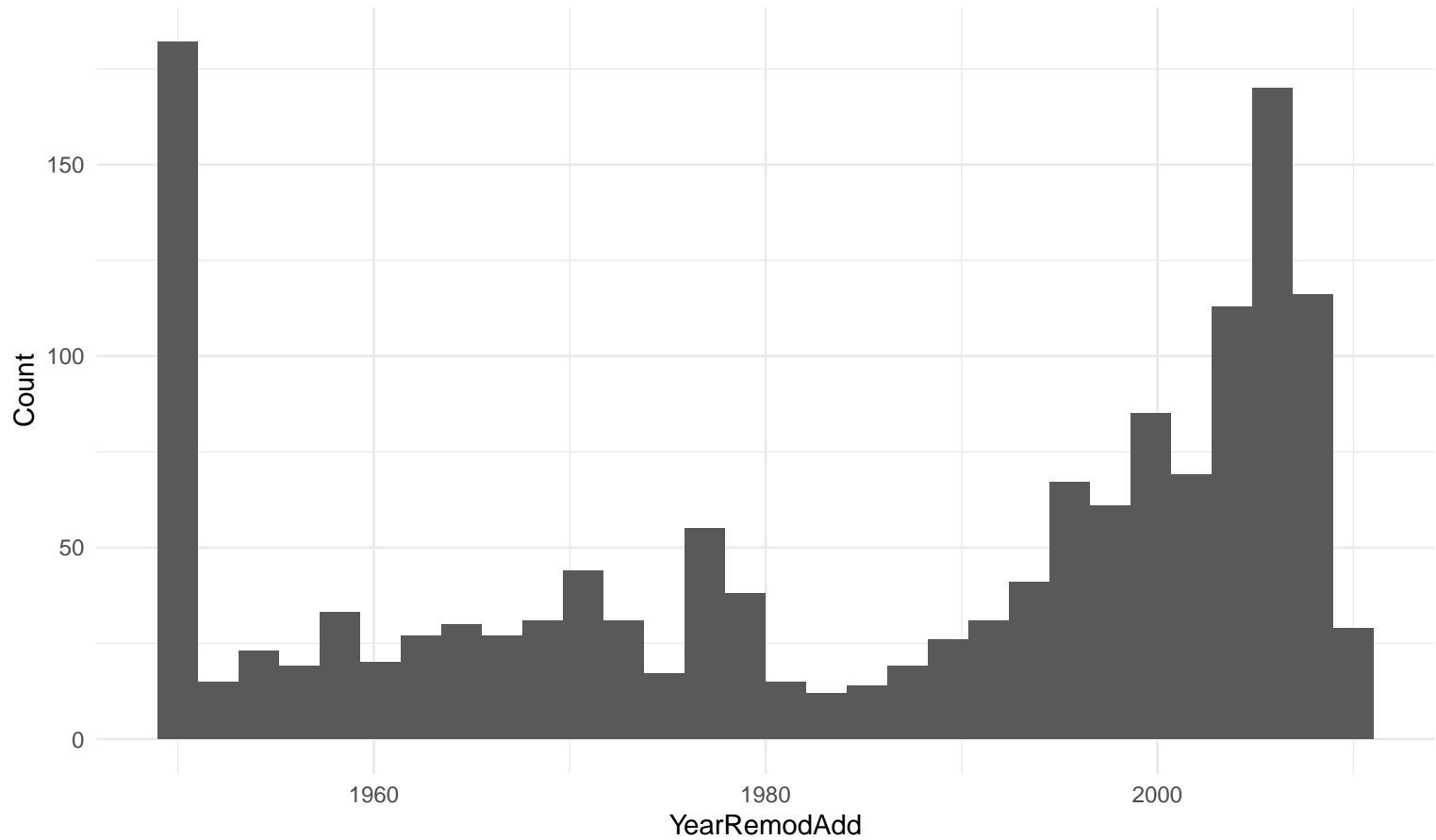
Histogram: YearRemodAdd
