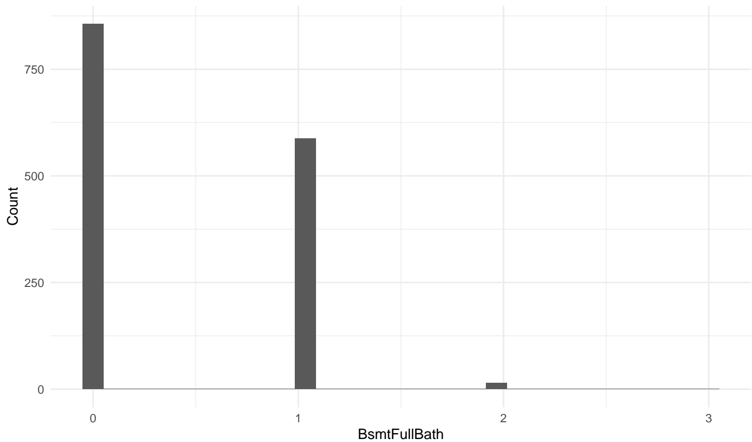
Histogram: BsmtFullBath
