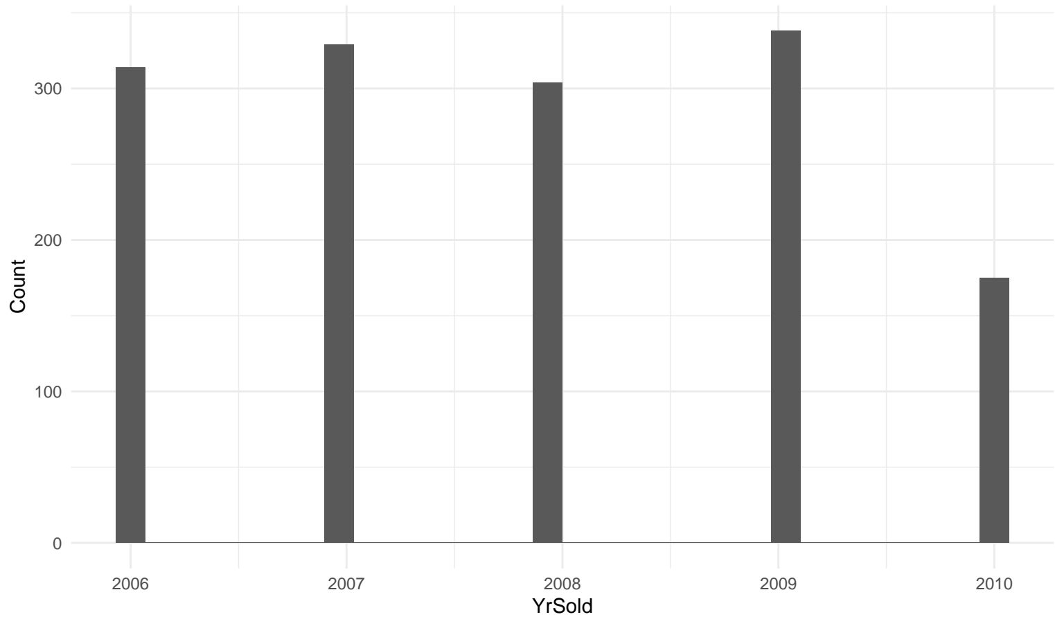
Histogram: YrSold
