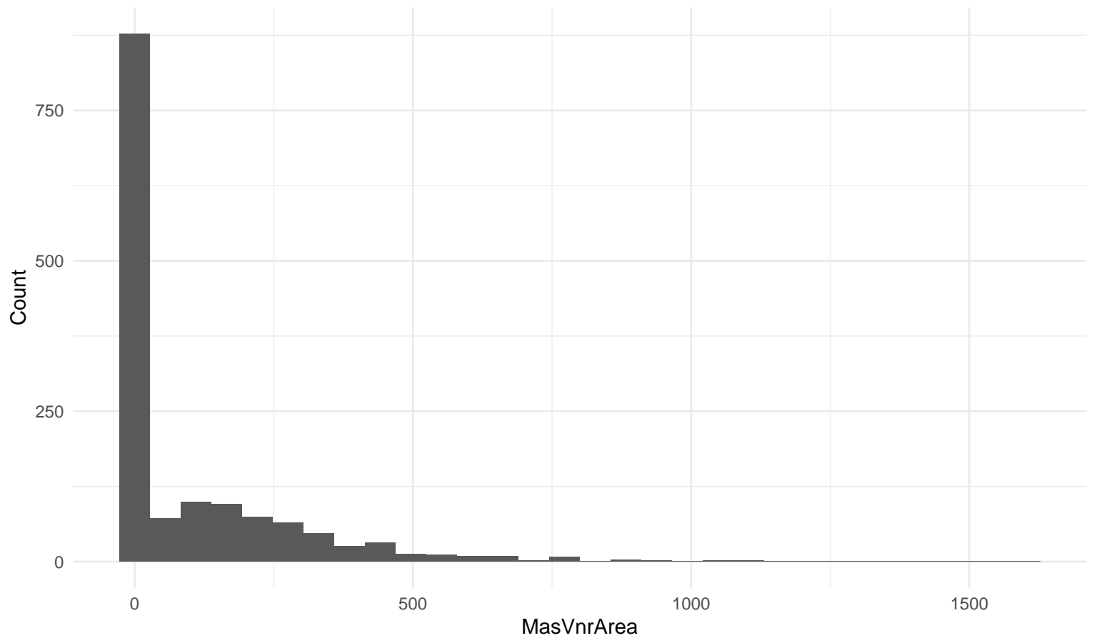
Histogram: MasVnrArea
