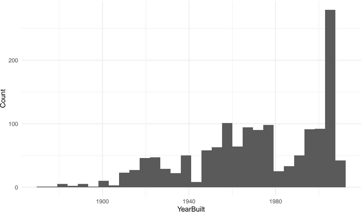
Histogram: YearBuilt
