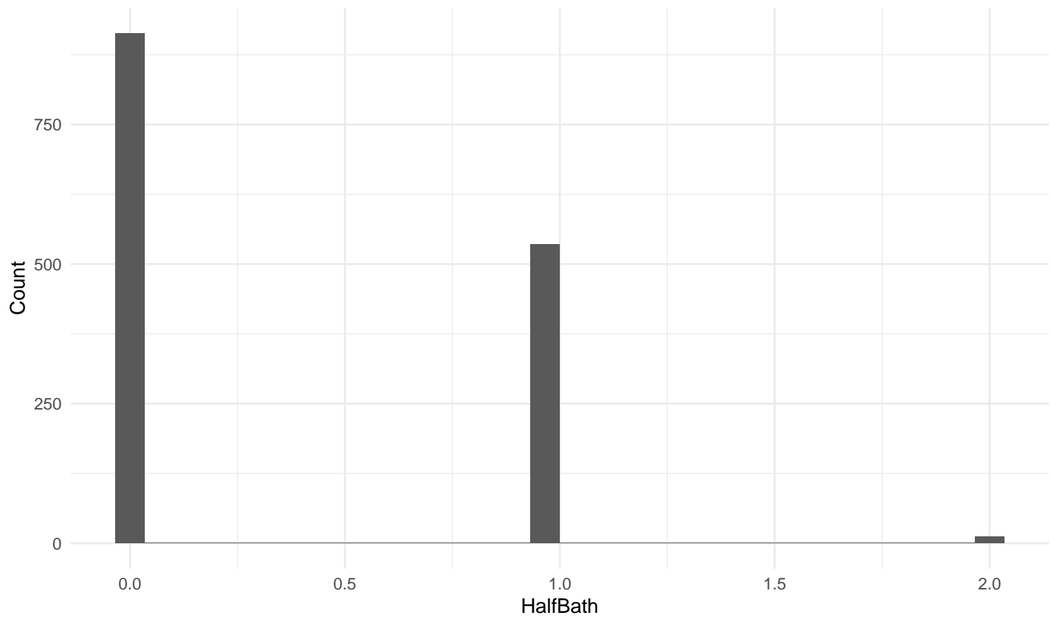
Histogram: HalfBath
