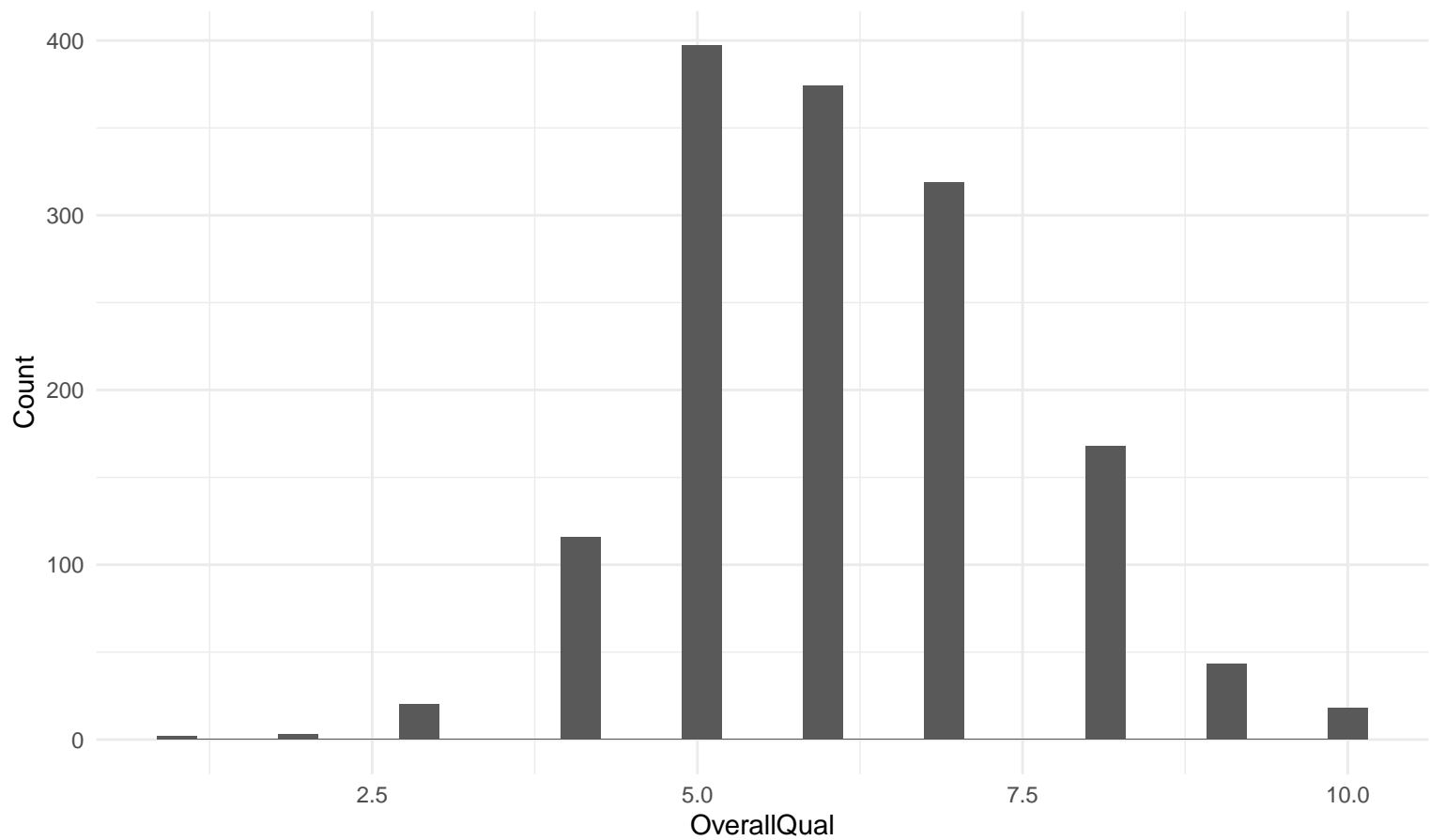
Histogram: OverallQual
