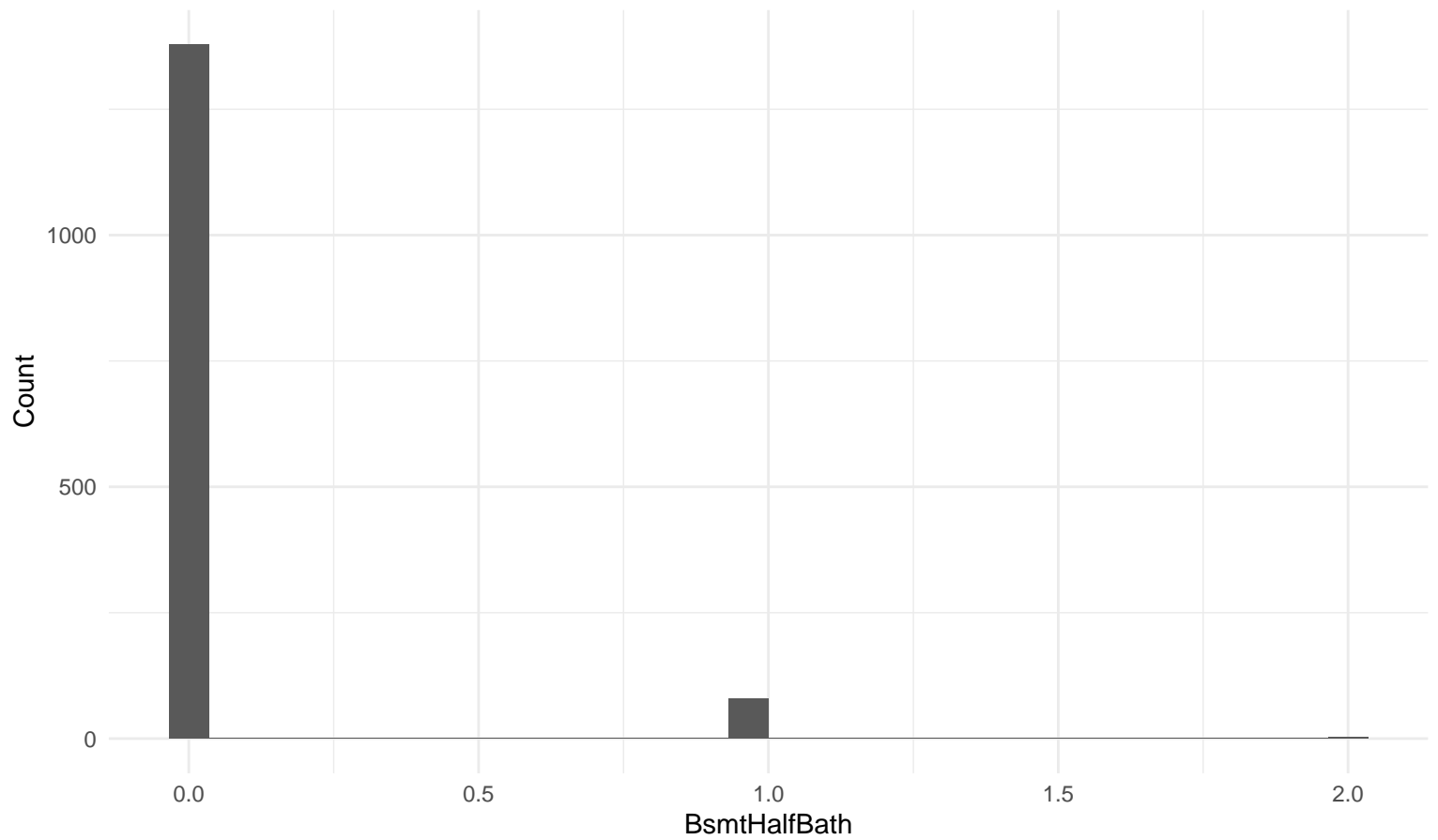
Histogram: BsmtHalfBath
