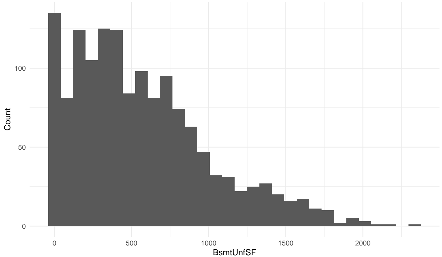
Histogram: BsmtUnfSF
