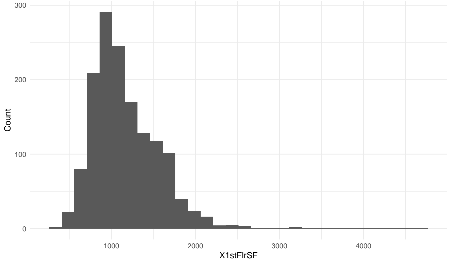
Histogram: X1stFlrSF
