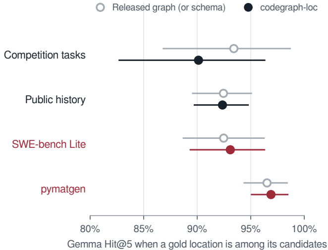
b Selection accuracy is the same with both graphs
