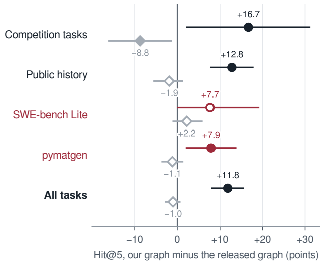
b The gain comes from code the released graph lacks
