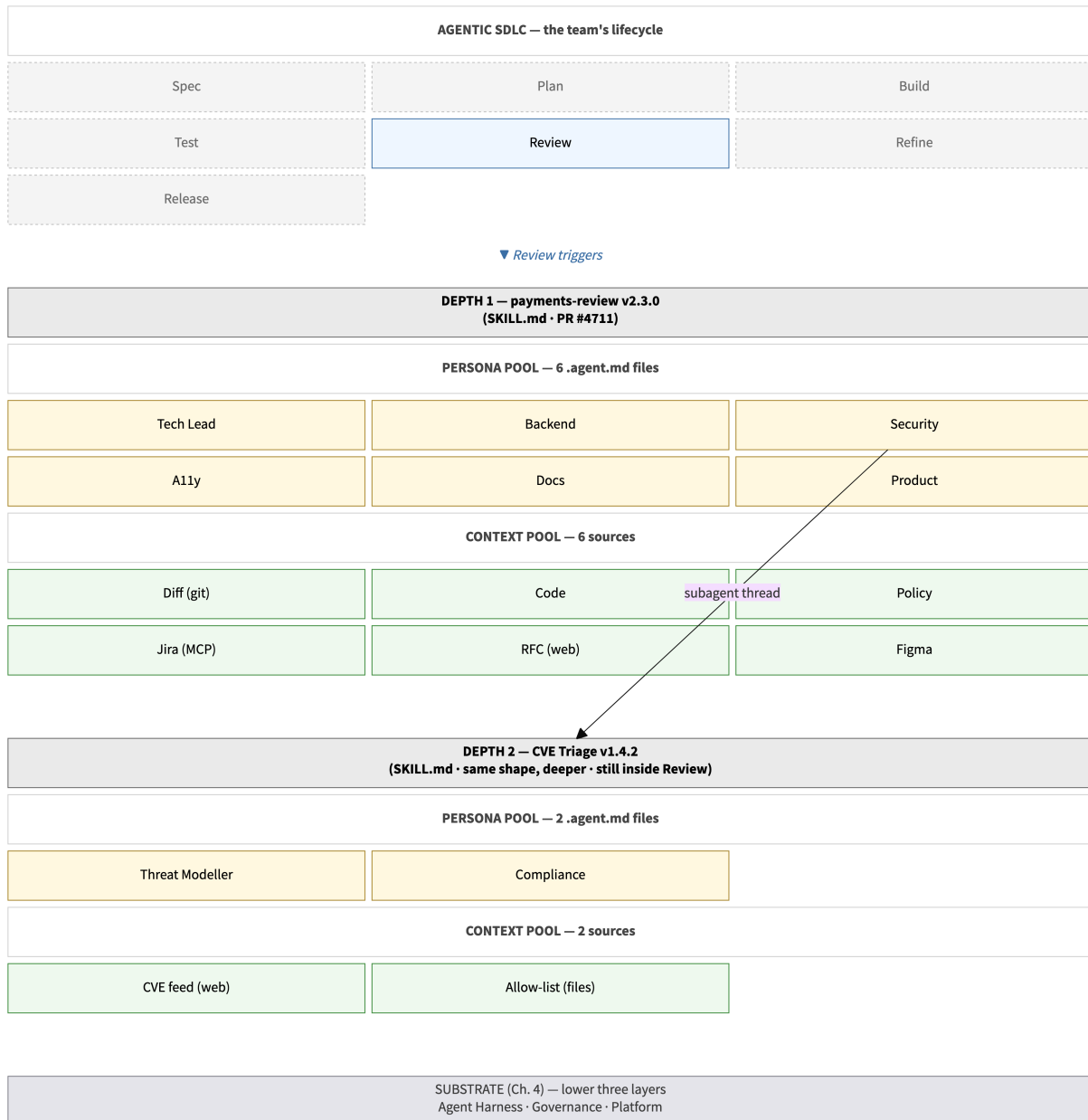
Figure 21.1: Maya's PR #4711. The team's Agentic SDLC sits at the top; the Review phase triggers the payments-review Skill, which dispatches Personas against Context. The same Skill→Persona→Context shape repeats at depth two when the Security Reviewer dispatches CVE Triage inside the same Review phase.
