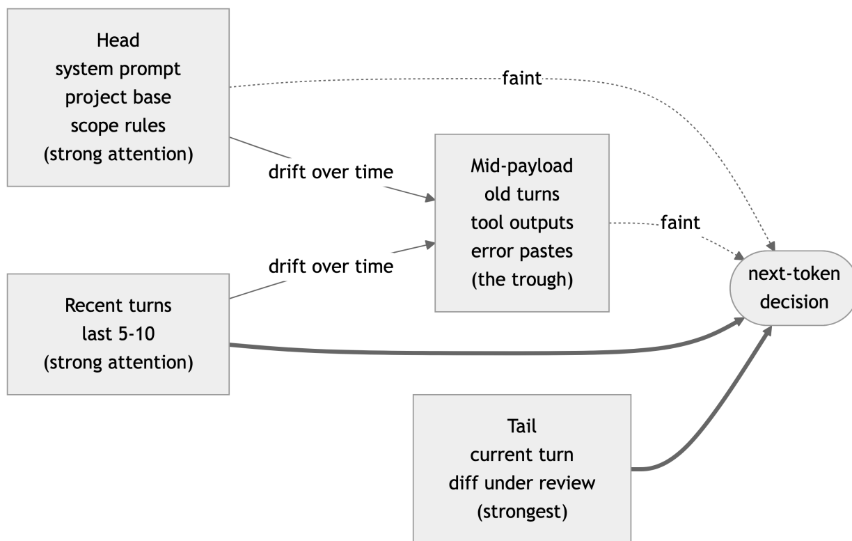
Figure 15.1: Position-by-time view of effective attention across a long agent session. Content near the head and tail of the context window receives strong attention; content in the middle is degraded; content that has slipped out of recent turns into mid-payload is taxed twice.
