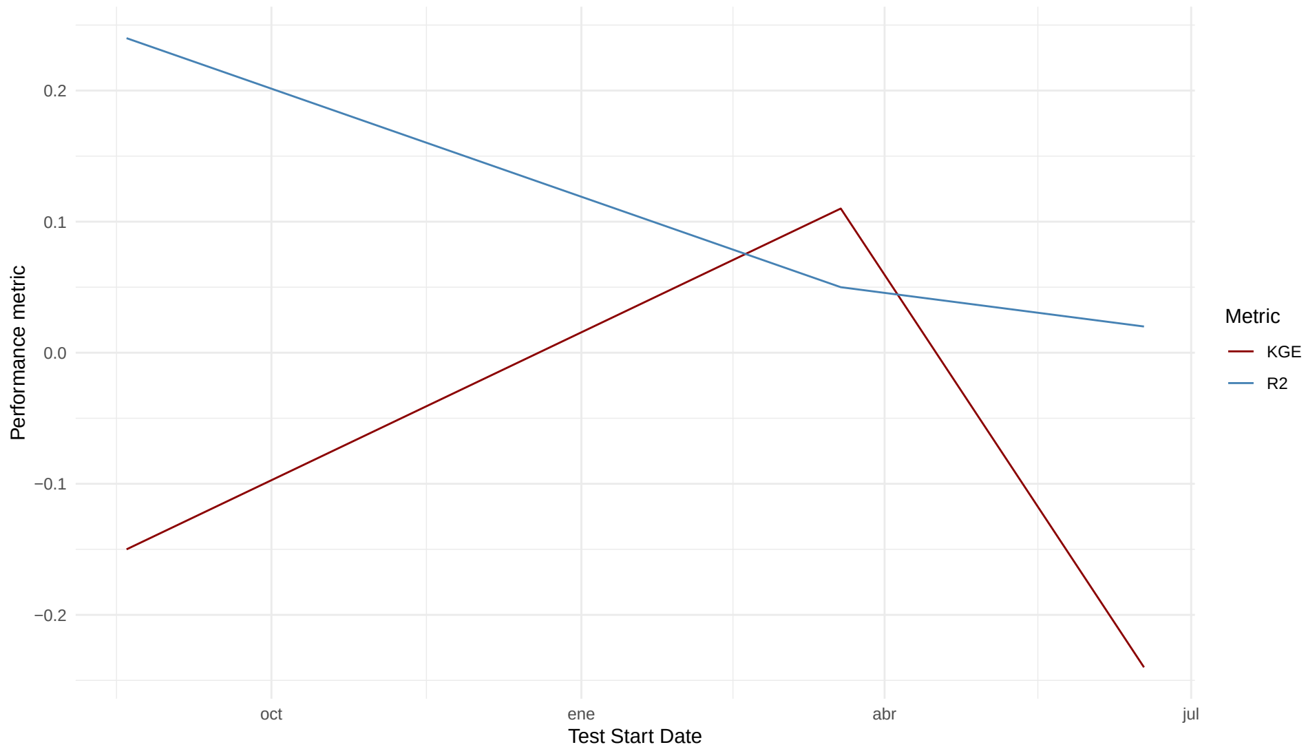
Rolling-window validation
