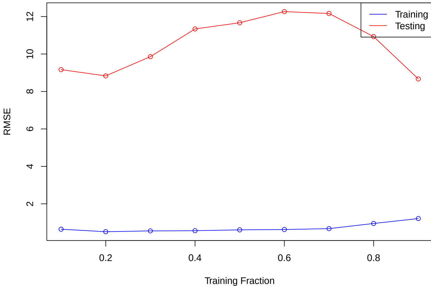
Learning Curve
