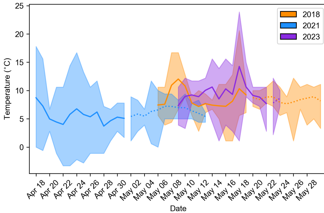
Fig. S14. Daily temperature time series for Yakutat Airport (10 m a.s.l.). Solid line is the daily mean, with the dotted lines being the daily mean during airborne data acquisition. Shading ranges between the daily minimum and maximum temperature.
