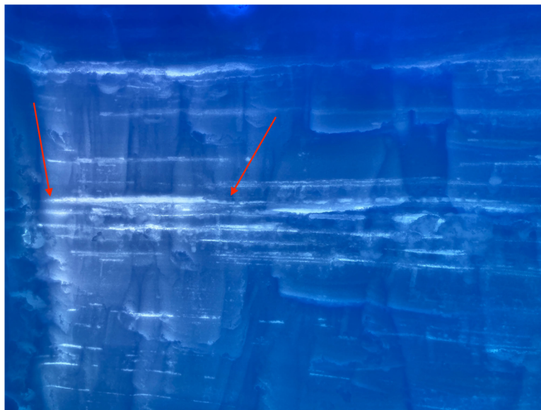
Fig. S12. Upper section of Snow Pit 1. Photo was taken by digging two adjacent snow pits with a preserved snow wall between them. The blue color is due to a blue tarp covering the snow pit. The ice layers were much more apparent through the snow wall than looking at the wall of a single snow pit. Red arrows in Figs. S12 and S13 are the same ice lens.
