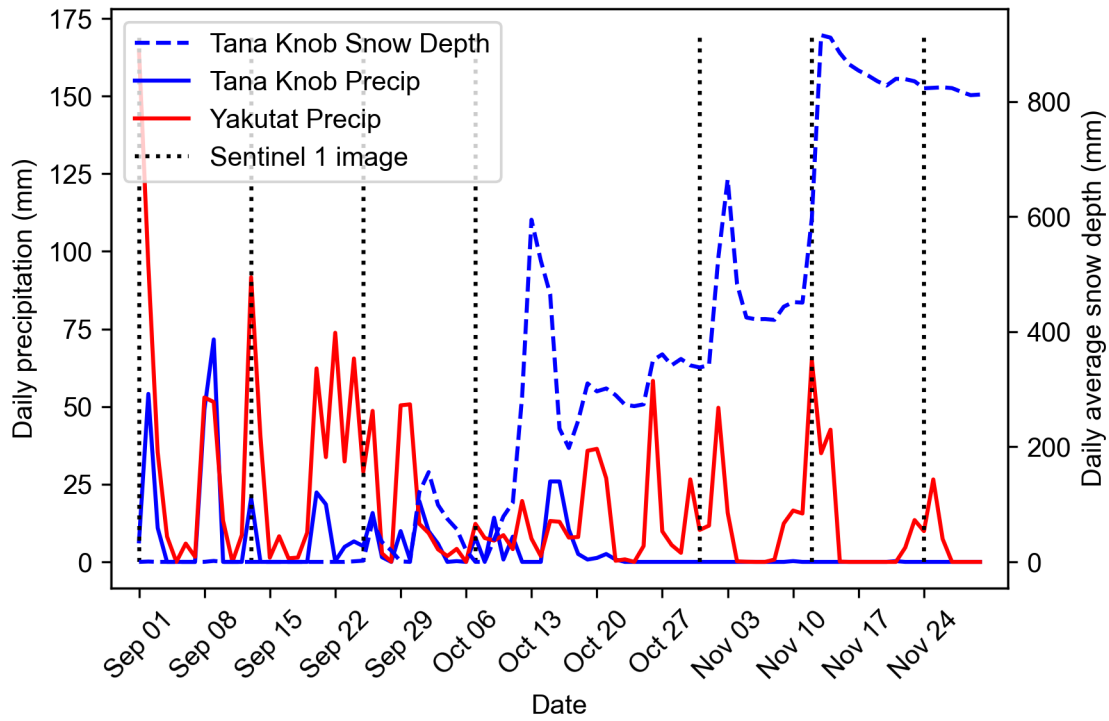
Fig. S16. Daily precipitation total (solid lines) for Tana Knob and Yakutat and the daily mean snow depth (dashed line) at Tana Knob for September 1st through November 30th, 2022. The lack of precipitation at Tana Knob after mid-October is likely due to no melt or liquid precipitation. The vertical dotted lines mark days when Sentinel 1 imagery was collected for the selected path and frame. There was no mid-October, 2022 image for the selected path and frame.
