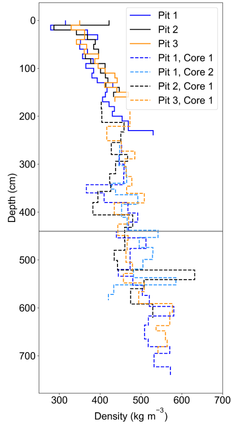
Fig. S11. Measured densities for the pits (solid lines) and cores (dashed). We omit the 9% uncertainty on each measurement in the plot for ease of seeing the measured value. Discontinuities at the pit to core interface are attributed to the change in sampling techniques. The gray horizontal line marks the approximate last summer surface depth.
