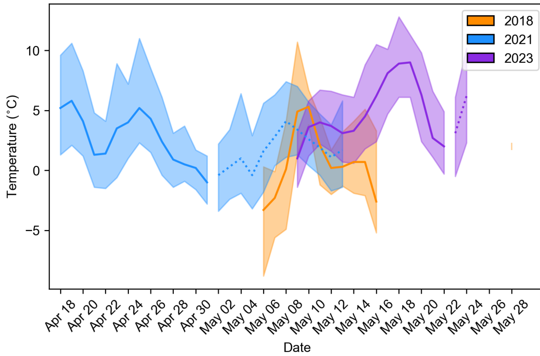
Fig. S15. Daily temperature time series for Tana Knob (1050 m a.s.l.). Solid line is the daily mean, with the dotted lines being the daily mean during airborne data acquisition. Shading ranges between the daily minimum and maximum temperature. Tana Knob was missing data in 2018, which is why there is less data coverage than compared to Yakutat (Fig. S14).
