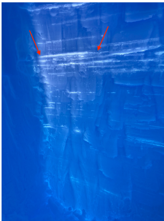
Fig. S13. Deeper section of Snow Pit 1, with the snow pit bottom in the lower left. After the concentration of ice layers shown in Fig. S12, they become less common deeper in the snow column.
