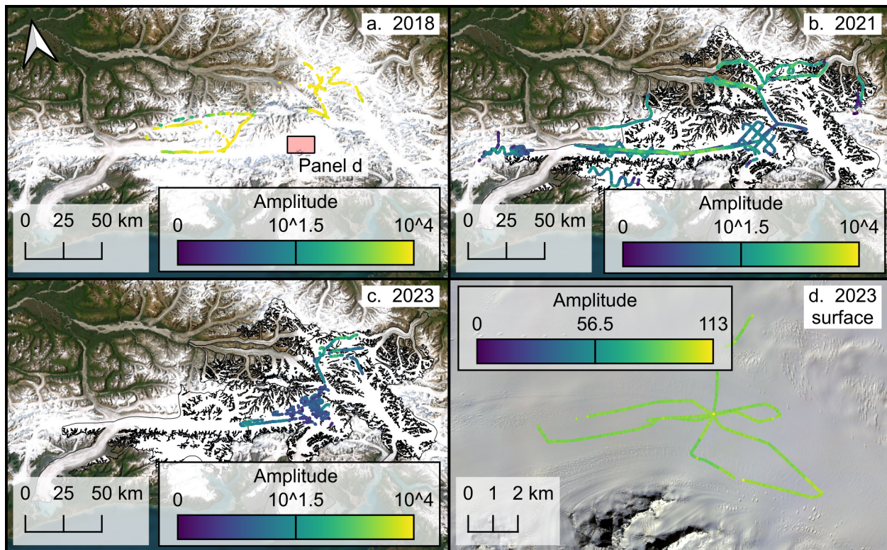
Fig. S19. Radar amplitude of the last summer surface for (a-c) the airborne radar and the (d) surface GPR. The scale for (a-c) the airborne radar is a logarithmic scale while the scale for the (d) surface GPR is a linear scale.
