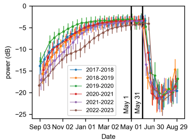
Fig. S18. Time series of Sentinel 1 reflectivity at the Kaskawulsh core site. Error bars are the one standard deviation of the power in the sampling area. Red line is the 2020-2021 accumulation season. No drop in reflectivity during fall 2020 is observed, which supports the interpretation of a strong, end of season ice layer that is not overlain by a fall rain on snow event. Also, the reflectivity drop from the onset of summer melting occurs later in the year than at the Seward sites due to the Kaskawulsh core site being at \sim 2650 m a.s.l., a kilometer higher than the Seward core sites.
