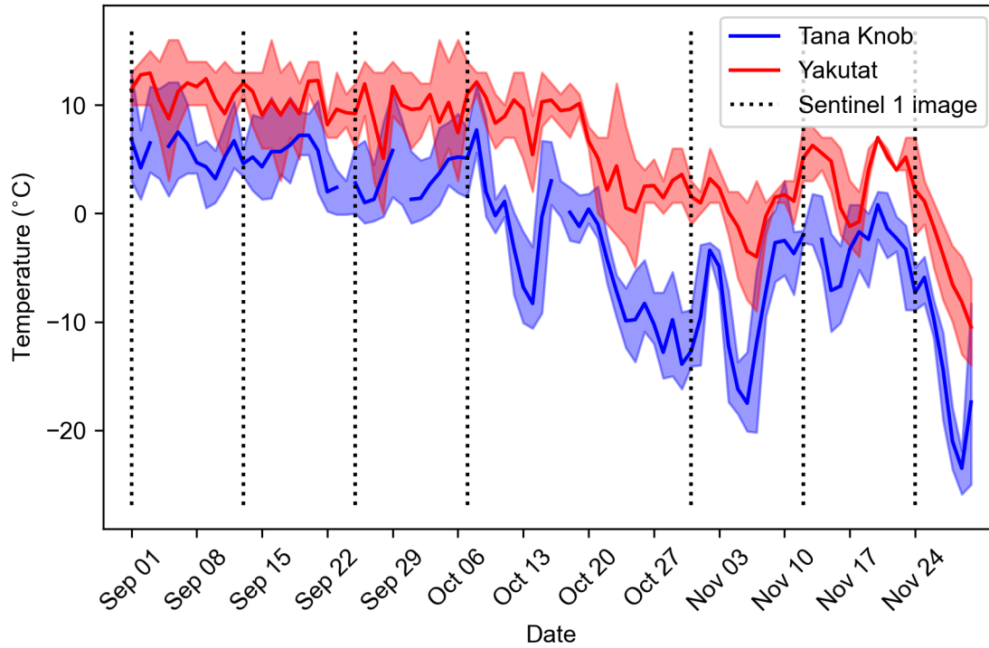
Fig. S17. Daily average temperature for Tana Knob and Yakutat for September 1st through November 30th, 2022. Shading ranges between the daily minimum and maximum. The vertical dotted lines mark days when Sentinel 1 imagery was collected for the selected path and frame. There was no mid-October, 2022 image for the selected path and frame.
