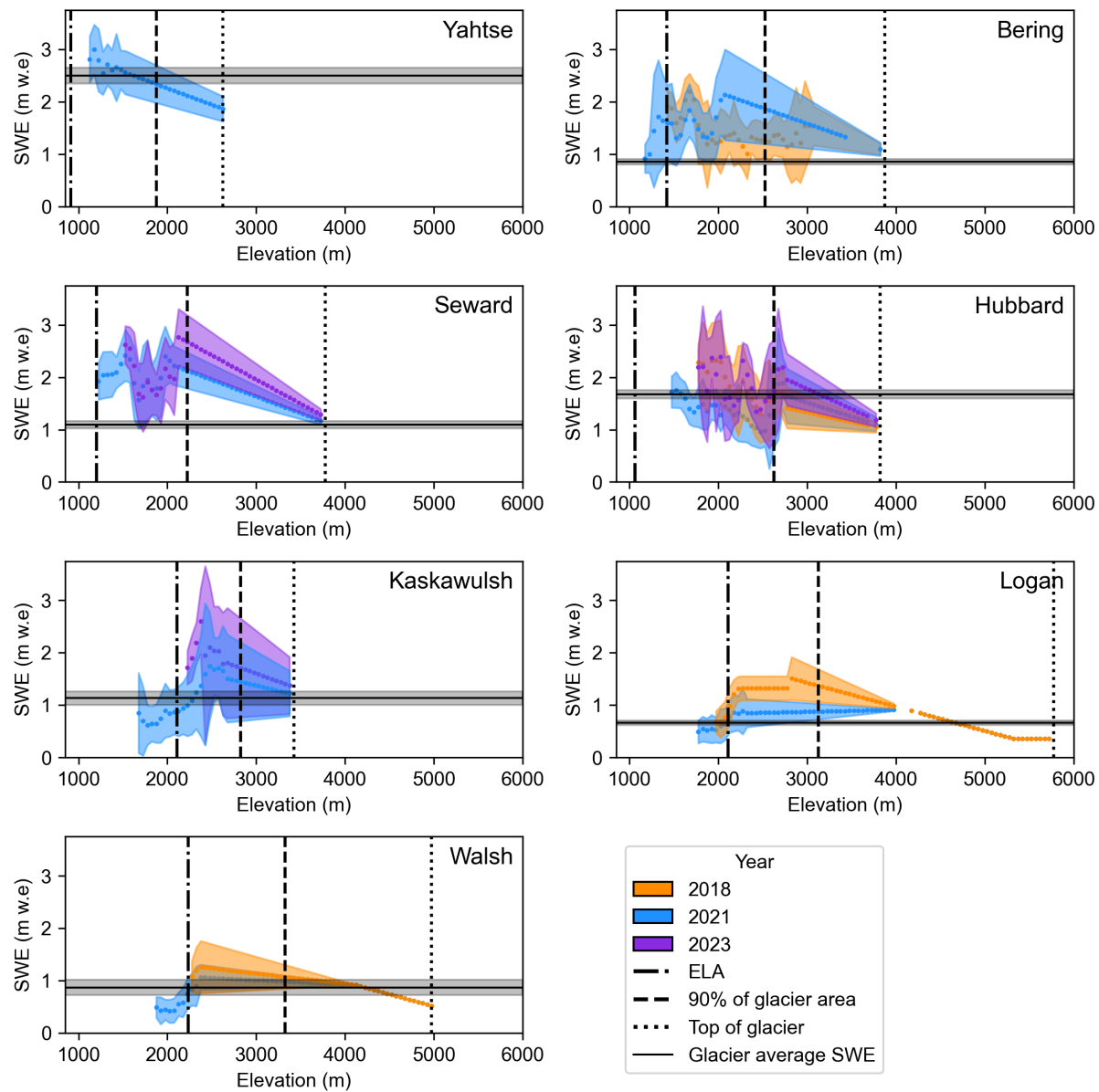
Fig. S7. SWE values for each elevation bin including the interpolation to the high elevation core sites on Mt. Logan. The glacier average SWE distributes the input mass to the accumulation area over the total glacier area, which causes the this value to be lower than most elevation bin values.
