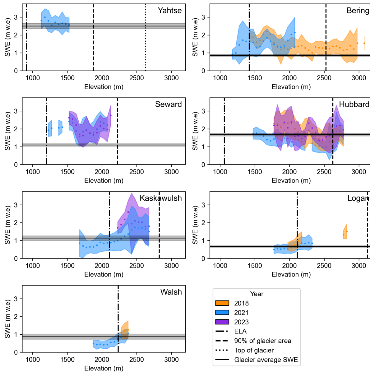
Fig. S8. SWE values for each elevation bin without the interpolation of missing data within elevations sampled by the airborne radar. Interpolation within the radar data only needed to be done of the Seward in 2021, Hubbard in 2021, and Logan in 2018. The glacier average SWE distributes the input mass to the accumulation area over the total glacier area, which causes the this value to be lower than most elevation bin values.
