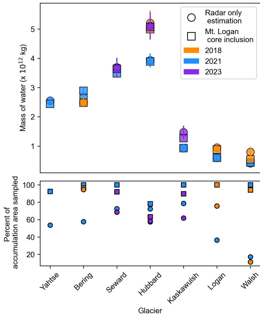
Fig. S9. (a) Winter mass balance in mass of water for each glacier by survey year and (b) corresponding percent of the accumulation area sampled. Glaciers are ordered roughly by their distance from the coast, closer (left) to further (right). Here we only show the uncertainties from the radar only estimation. In this plot we show only the 2\sigma uncertainty for the radar only estimation.
