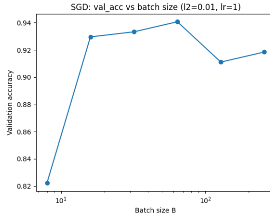
FIGURE 3. Validation accuracy vs. batch size for SGD
