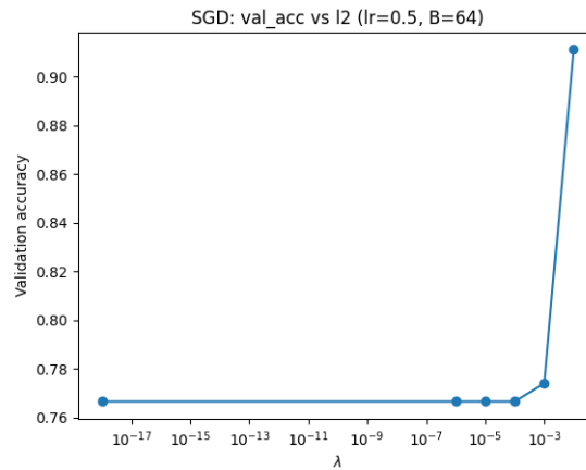
FIGURE 1. Final validation accuracy vs. L^2 regularization parameter for SGD
