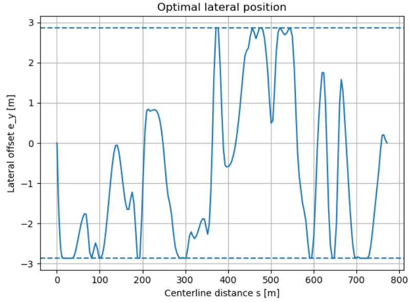
FIGURE 2. Optimized lateral displacement with admissible track limits.
