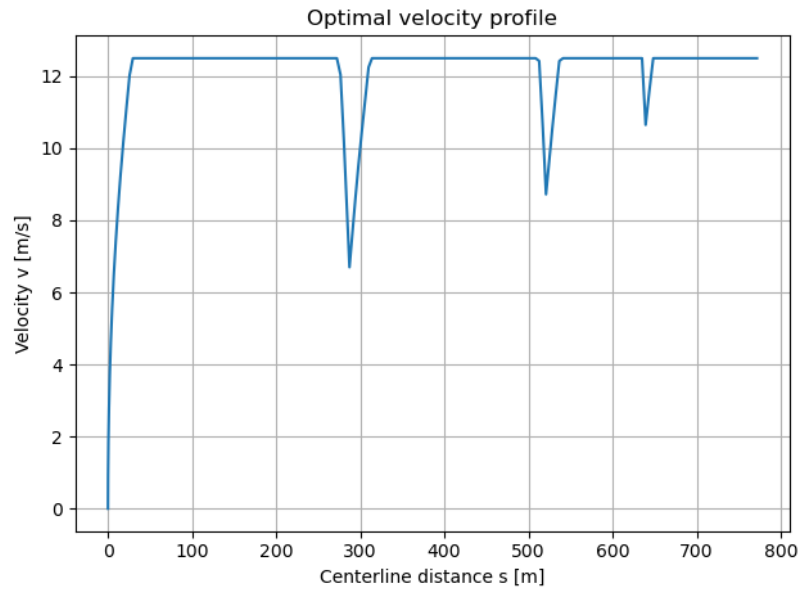
FIGURE 3. Optimal velocity profile along the track centerline.
