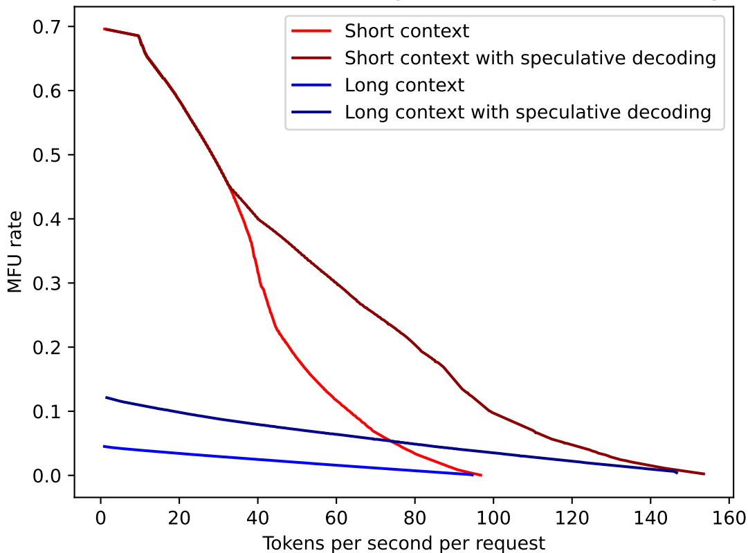
Token economics of Mistral Large 2 on different context lengths
