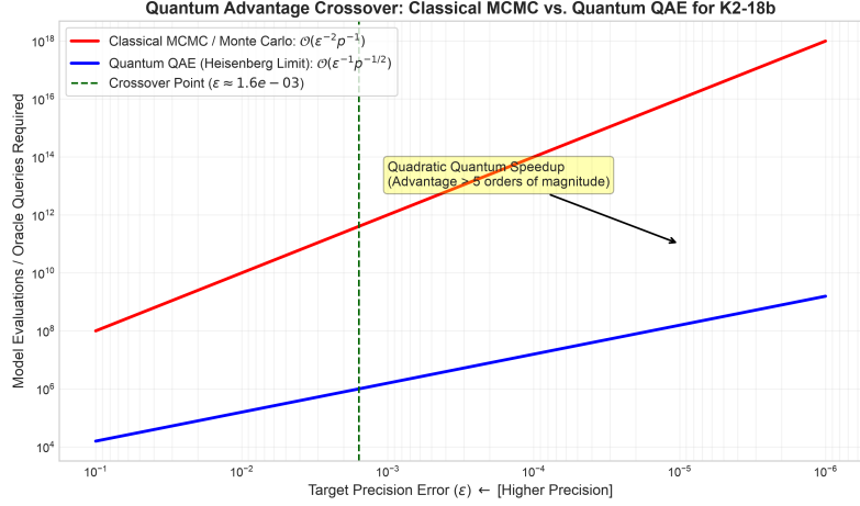
Figure 2.3. Quantum Advantage Crossover Point: Classical MCMC vs. Quantum QAE for Rare-Event Inference ( p = 10^{-6} ). Comparison of the required computational query volume as a function of target precision \epsilon . The classical stochastic method scales as \mathcal{O}(\epsilon^{-2}p^{-1}) , while Quantum Amplitude Estimation scales at the Heisenberg limit \mathcal{O}(\epsilon^{-1}p^{-1/2}) . The crossover occurs at \epsilon_{\text{cross}} \approx \frac{\pi}{2}\sqrt{p} \approx 1.57 \times 10^{-3} , beyond which the quantum pipeline delivers a computational advantage exceeding 5 orders of magnitude.
