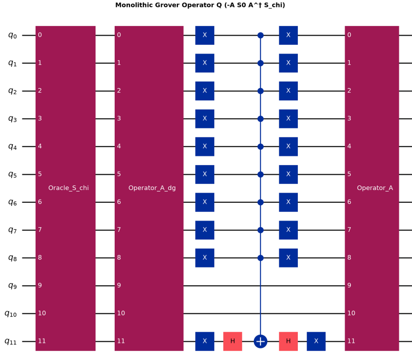
Figure 3.3. Quantum Circuit Architecture of the Grover Iteration Operator \mathcal{Q} . The operator executes a phase inversion of marked target states ( S_{\chi} ), followed by inverse state preparation ( A^\dagger ), zero-state phase reflection ( S_0 ), and forward state preparation ( A ), producing a deterministic 2\theta rotation in the bipartite plane.
