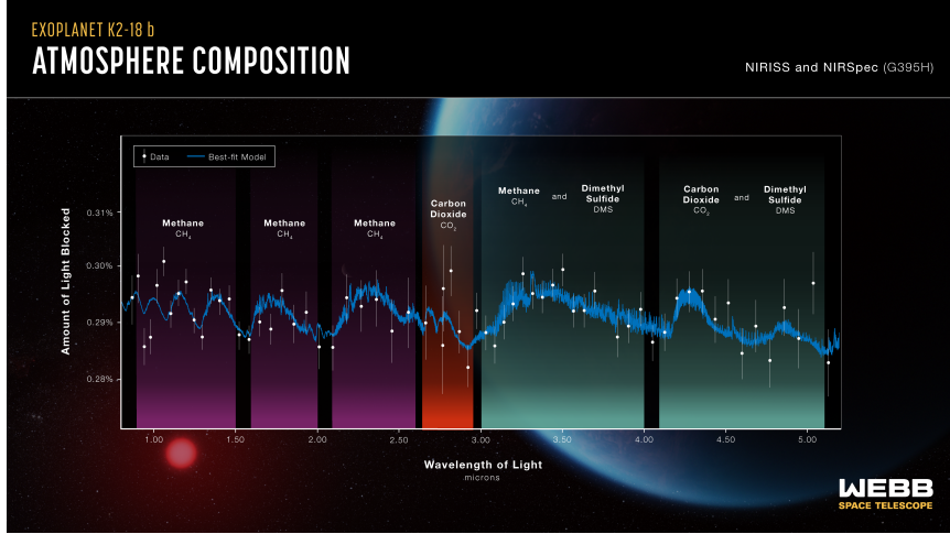
Figure 1.1. Transmission Spectrum of Exoplanet K2-18b (JWST NIRISS & NIRSpec). The observational data reveal prominent absorption features of carbon-bearing molecules ( \text{CH}_4 and \text{CO}_2 ) while showing a depleted abundance of \text{H}_2\text{O} and \text{NH}_3 . These spectral lines form the empirical baseline evidence for the astrobiological Bayesian inference model. Image credit: NASA/ESA/CSA/STScI.
