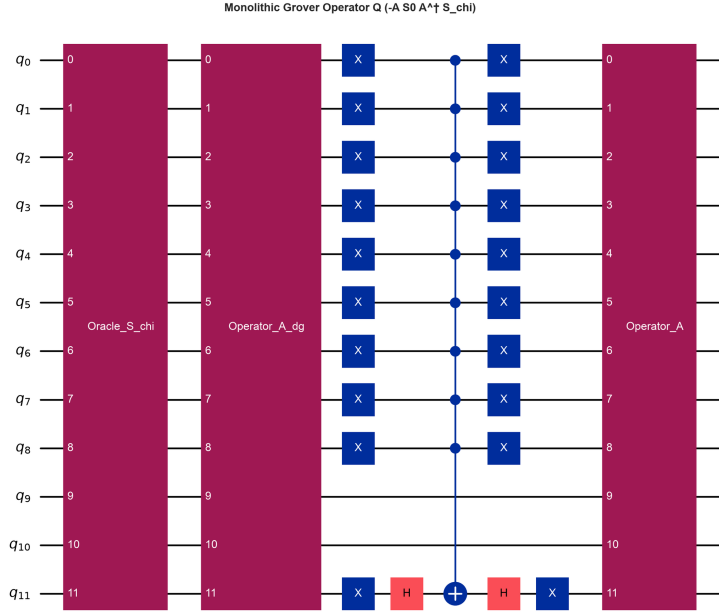
Figure 3.3. Quantum Circuit Architecture of the Grover Iteration Operator Q . The operator executes a phase inversion of marked target states ( S_{\chi} ), followed by inverse state preparation ( A^\dagger ), zero-state phase reflection ( S_0 ), and forward state preparation ( A ), producing a deterministic 2\theta rotation in the bipartite plane.
