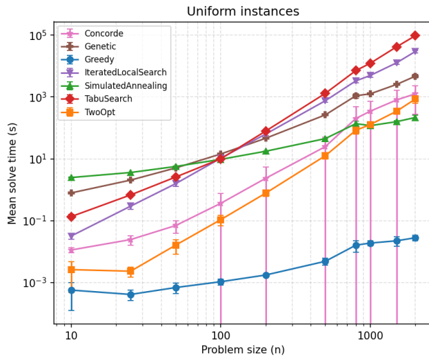
Fig. 4. Time scaling of uniform instances for different sizes and distributions.
