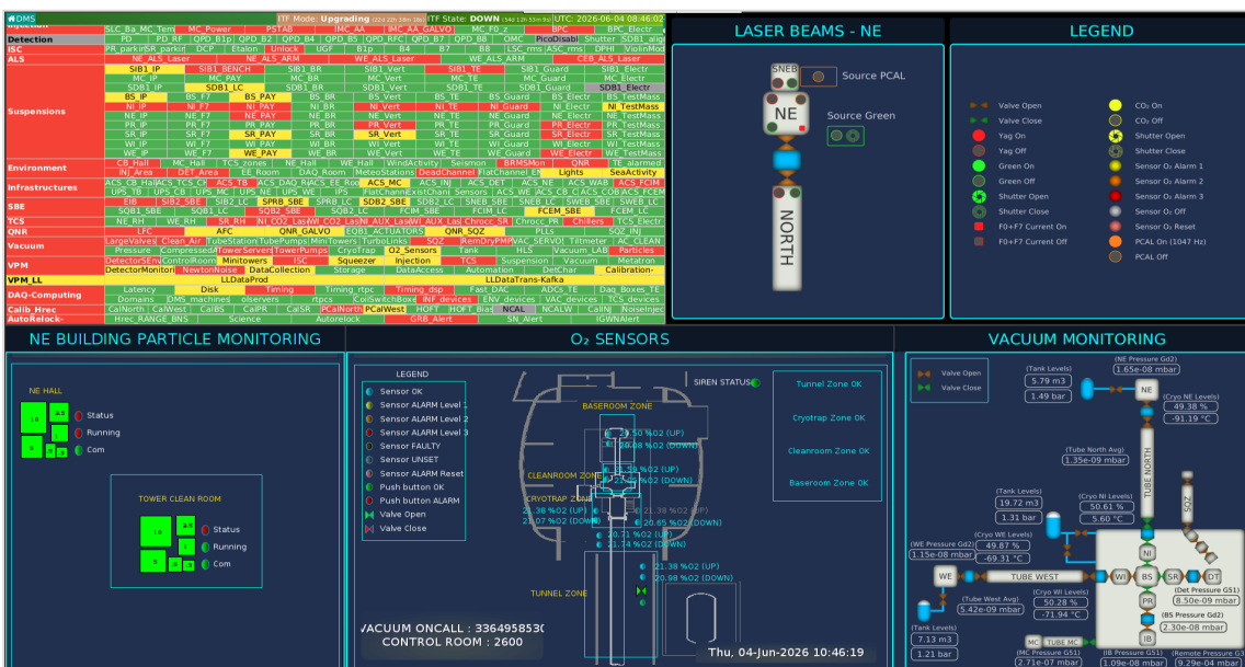
Figure 4 — North End local panel: NE O 2 sensors, NE Laser Beams diagram (Source Green, SNEB, tube toward CB), NE vacuum monitoring and the NE clean-room particle counters.
