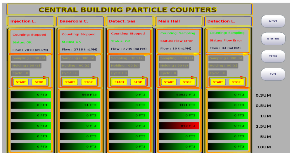
Figure 6 — Detailed view: five CB fixed counters with per-size absolute readings, alarms colour-coded green / red, and rack-level navigation buttons
