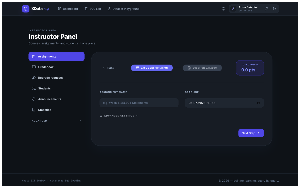
Figure 12: Creating an assignment: a two-step wizard — base configuration (name, deadline) then the question catalogue.
