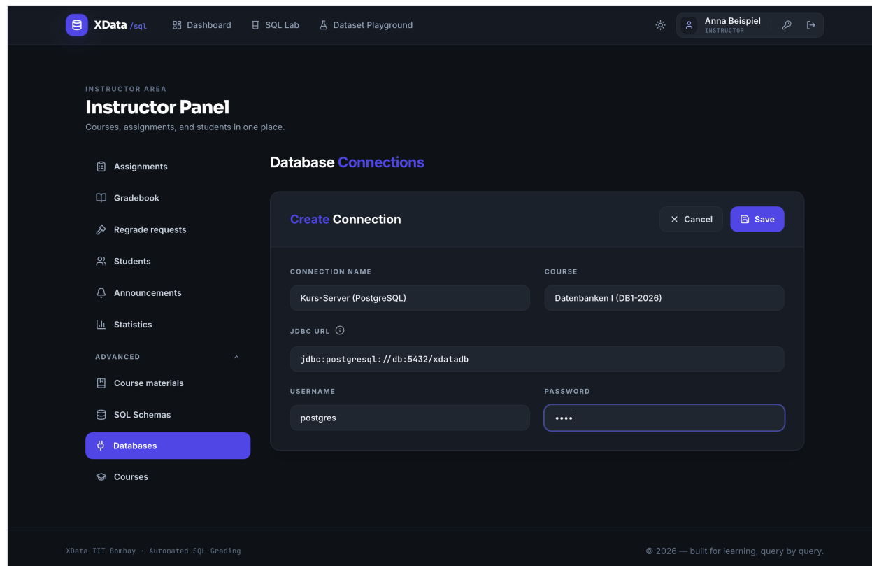
Figure 11: Creating a connection: name, course, JDBC URL, username and password.
