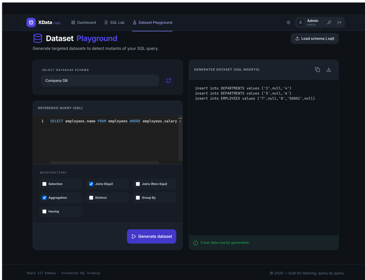
Figure 26: Mutation types are applied live: unticking a type removes its targeted rows from the generated dataset.
