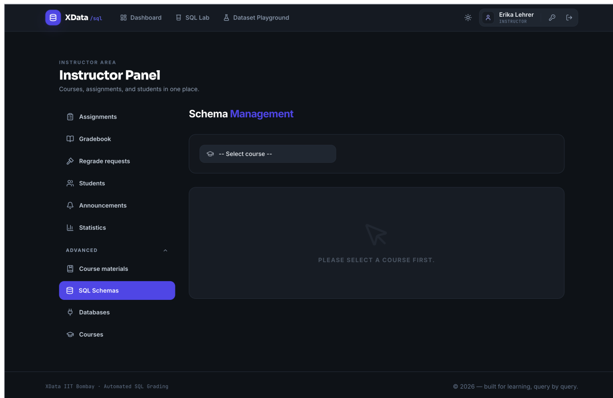
Figure 9: Schema management. Select a course, then create or edit the SQL schema used by its questions.
