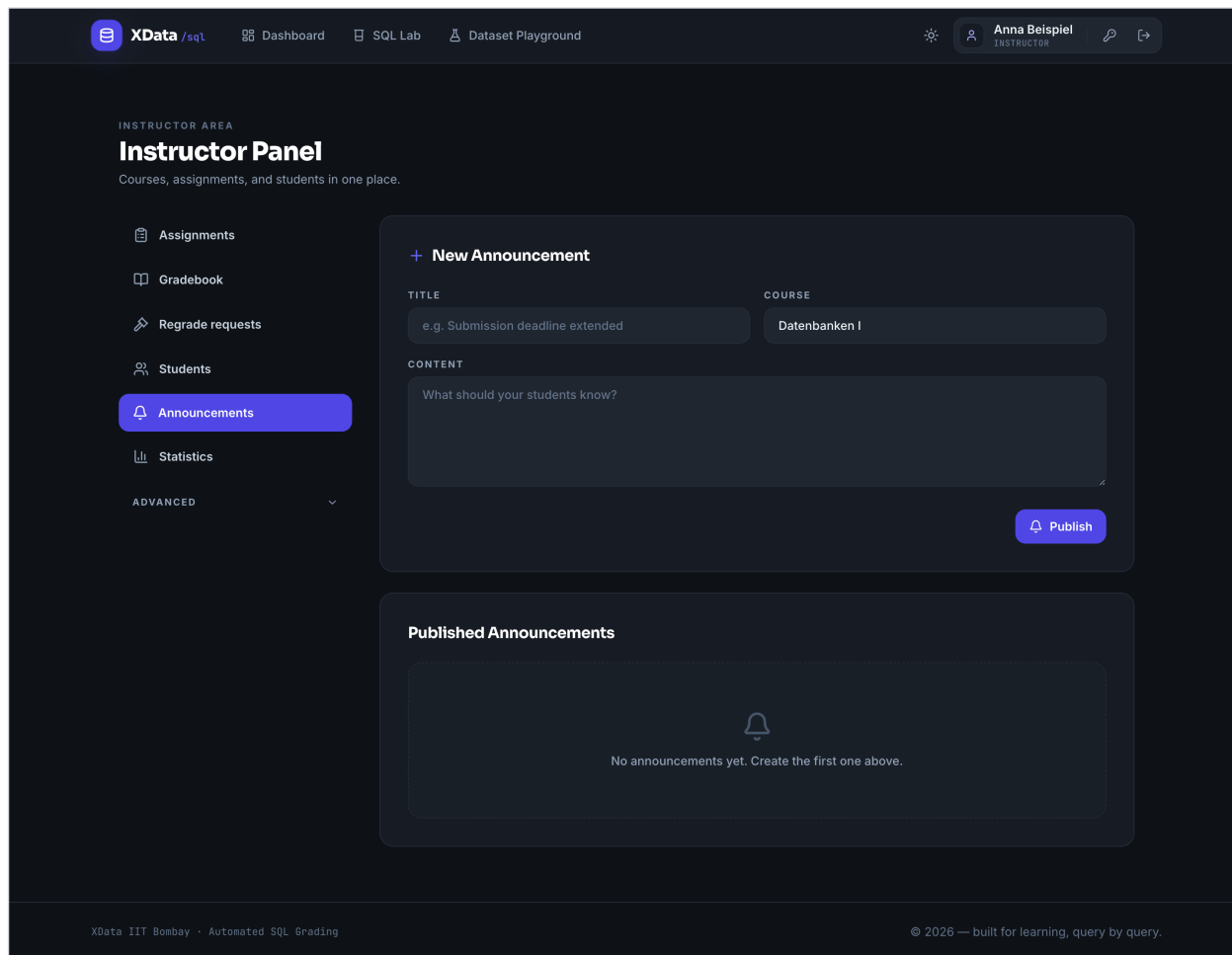
Figure 15: Announcements: post a message (title, course, content) to a course; published announcements are listed below.
