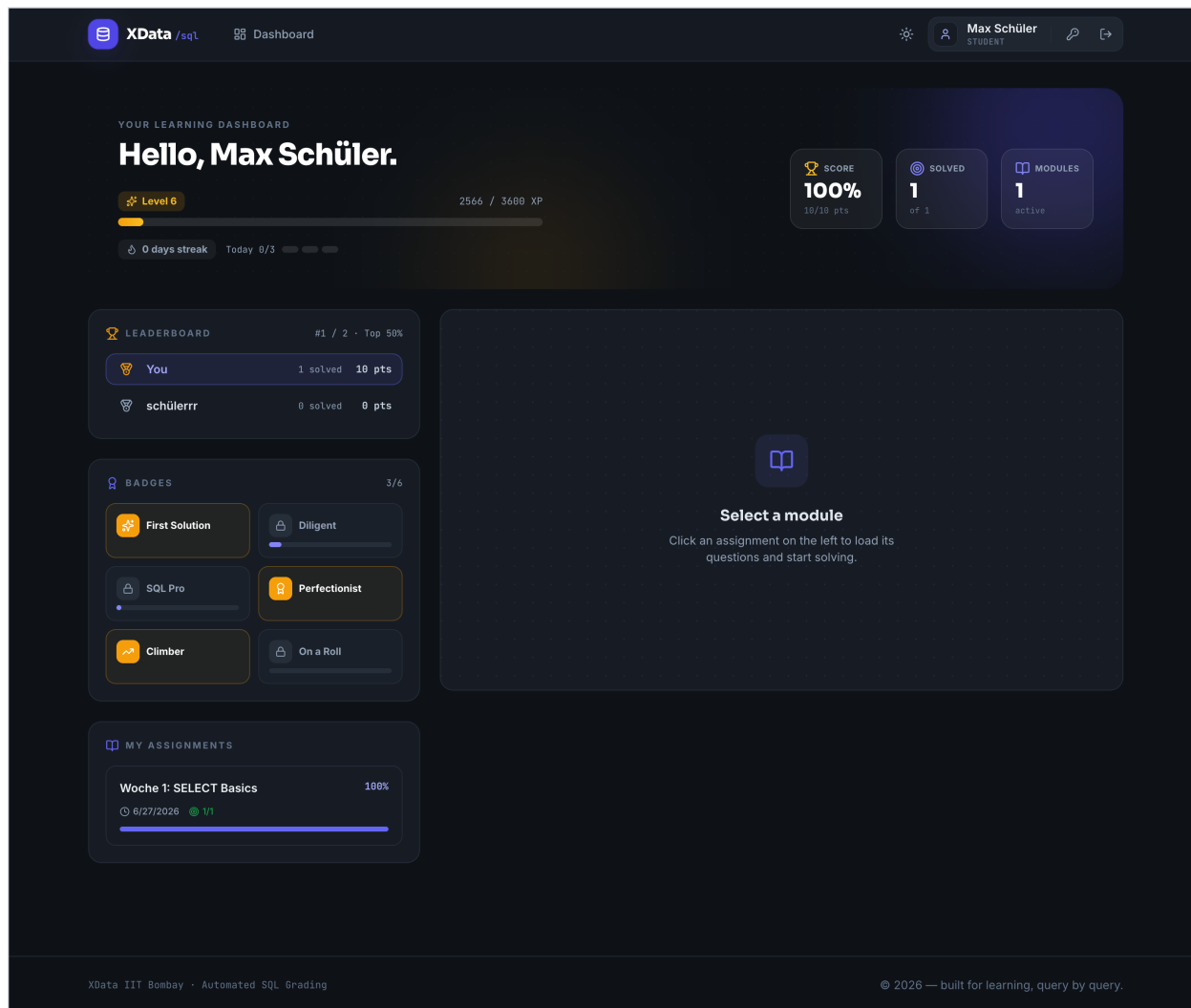
Figure 17: The student dashboard: XP and level, leaderboard, badges and assigned modules.
