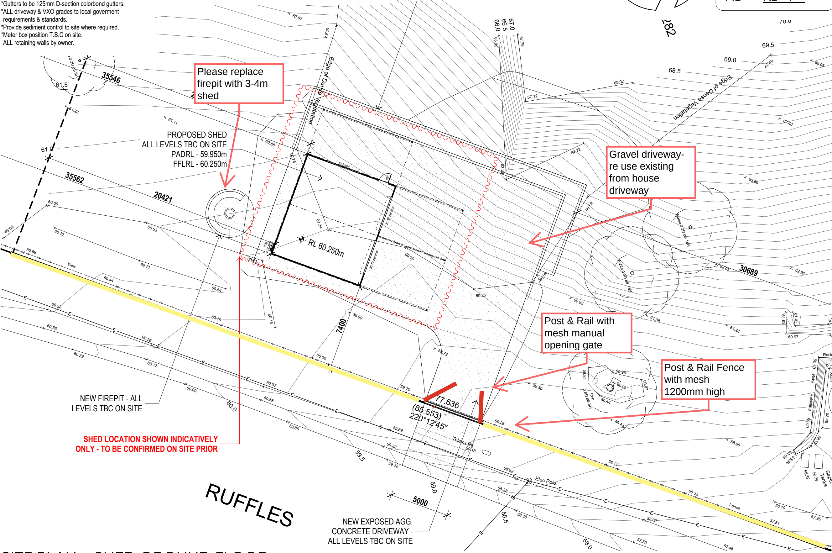
SITE PLAN – SHED GROUND FLOOR SCALE 1:200 SHEET 7 OF 24 JOB NUMBER – 10588
