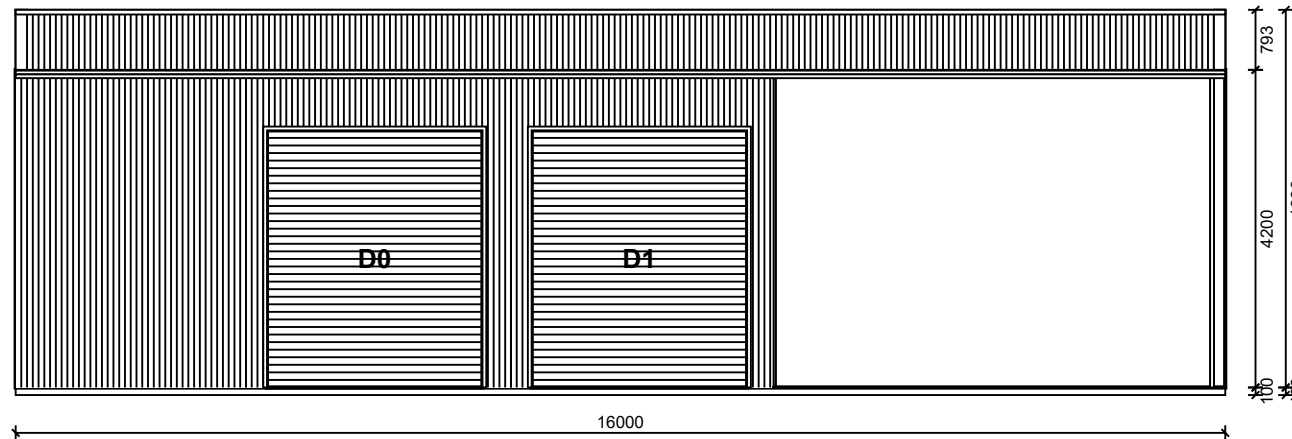
4. LEFT ELEVATION SCALE 1:100
