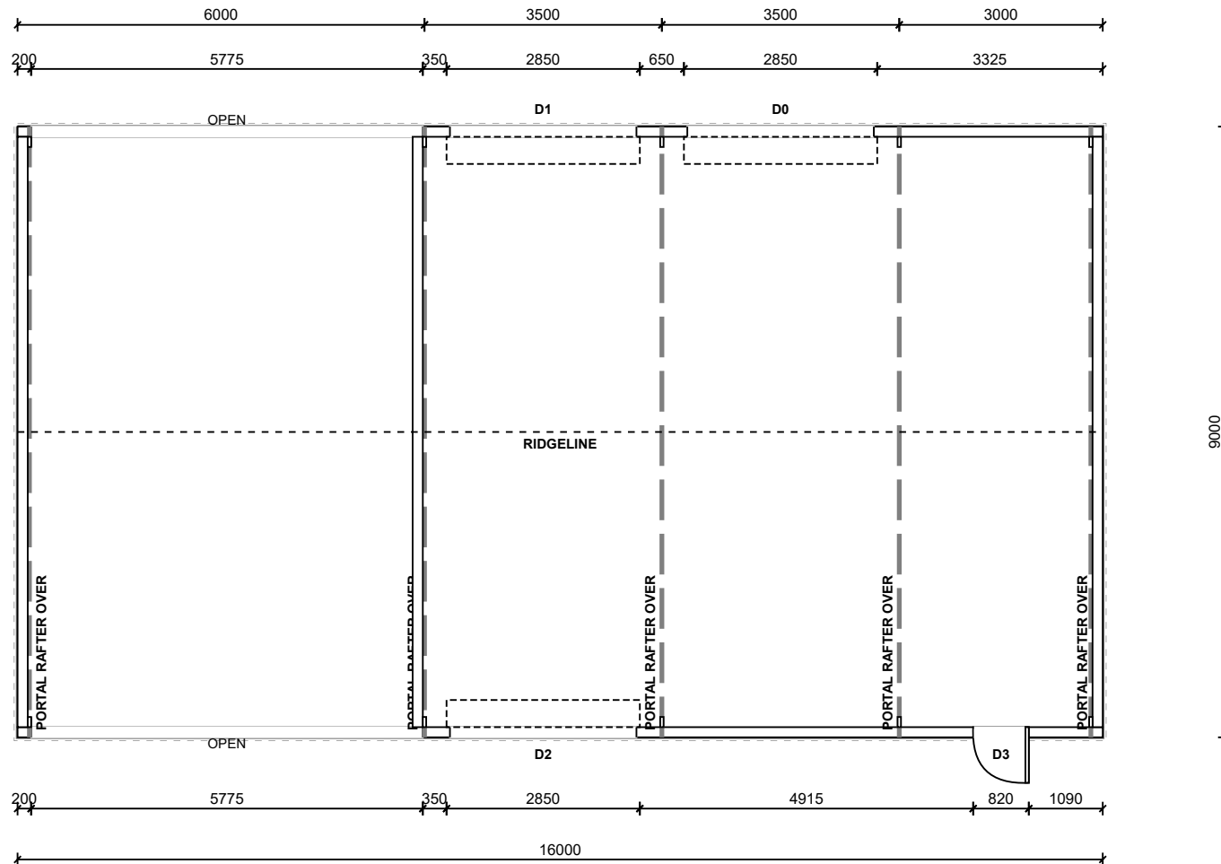
FLOORPLAN SCALE 1:100
