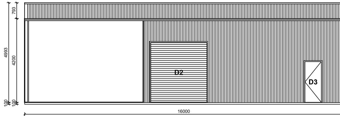
2. RIGHT ELEVATION SCALE 1:100
