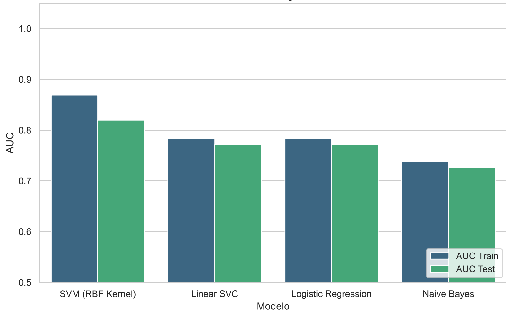
Análisis de Overfitting: Train vs Test
