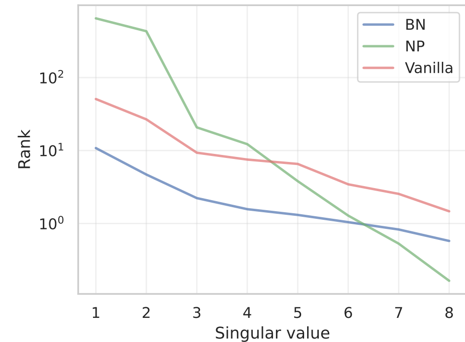
CIFAR-10 (small)
