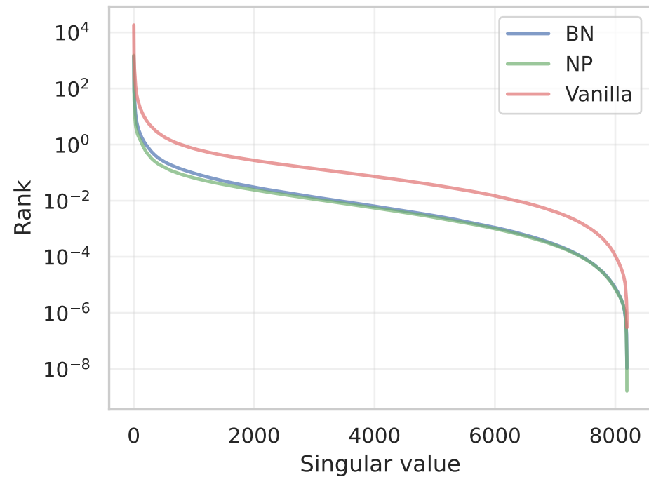
CIFAR-10
