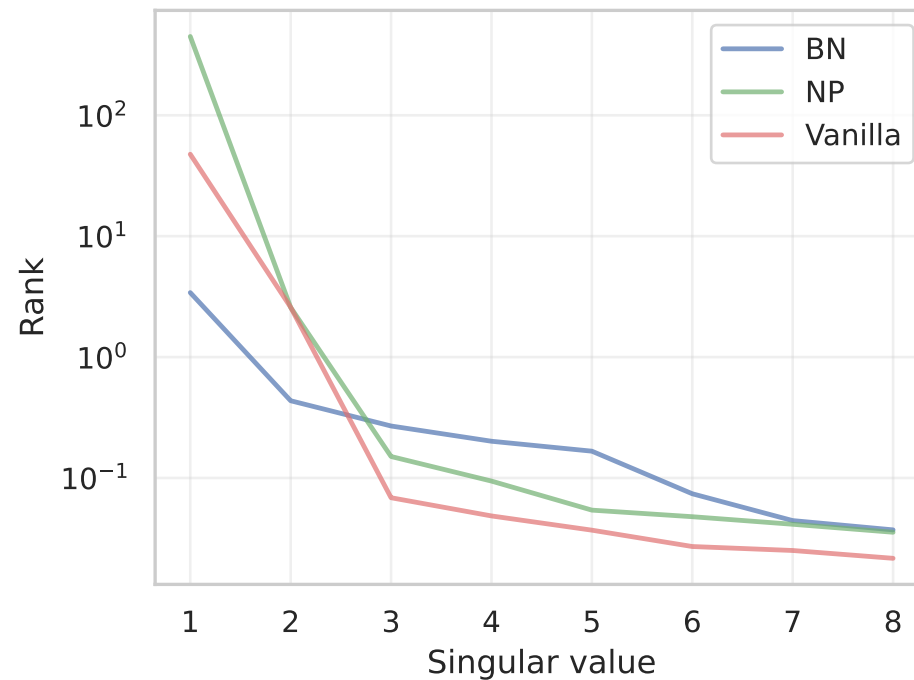
IMDb (small)
