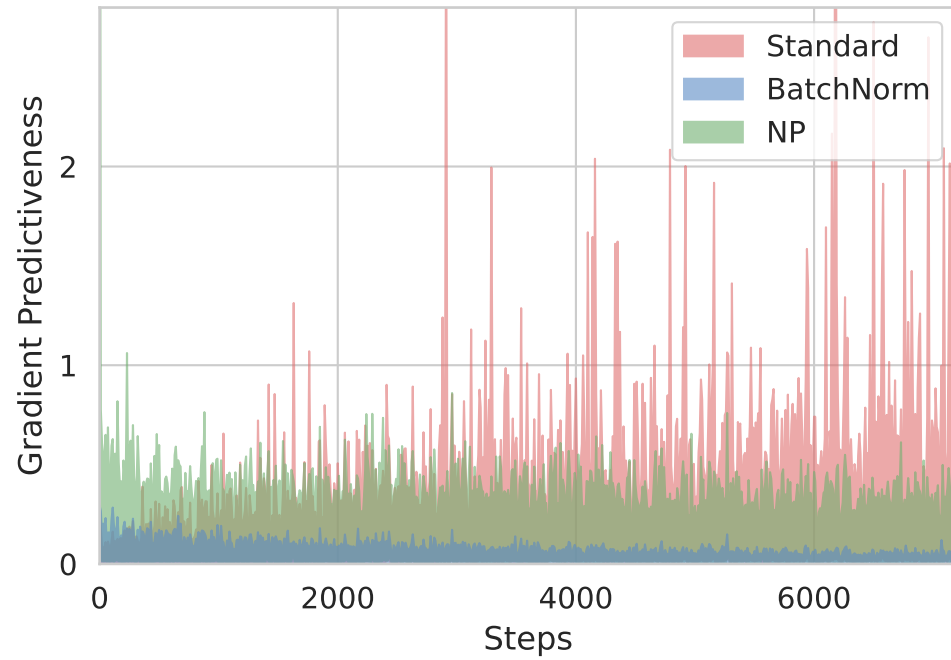
(b) Gradient Predictiveness
