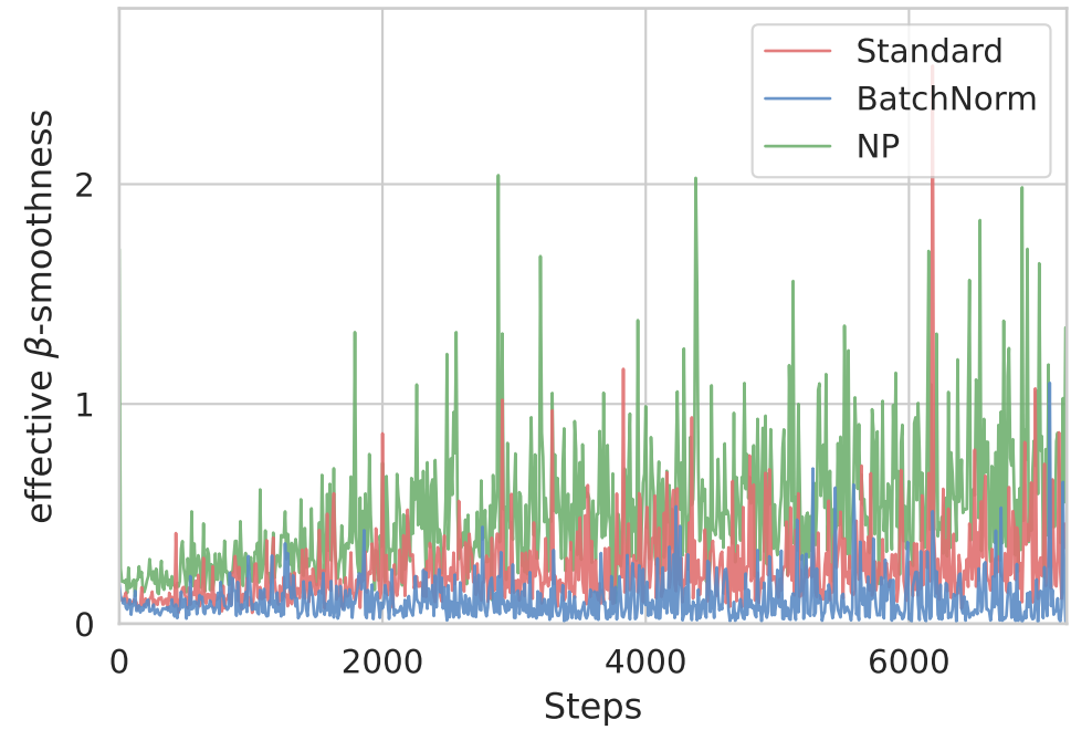
(c) Effective \beta -smoothness
