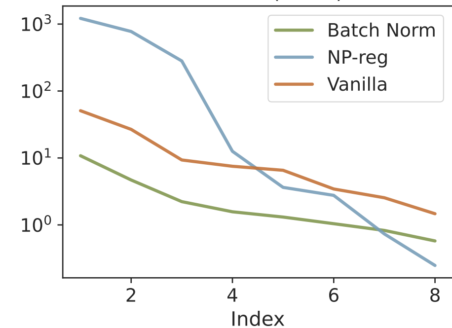
CIFAR-10 (small)
