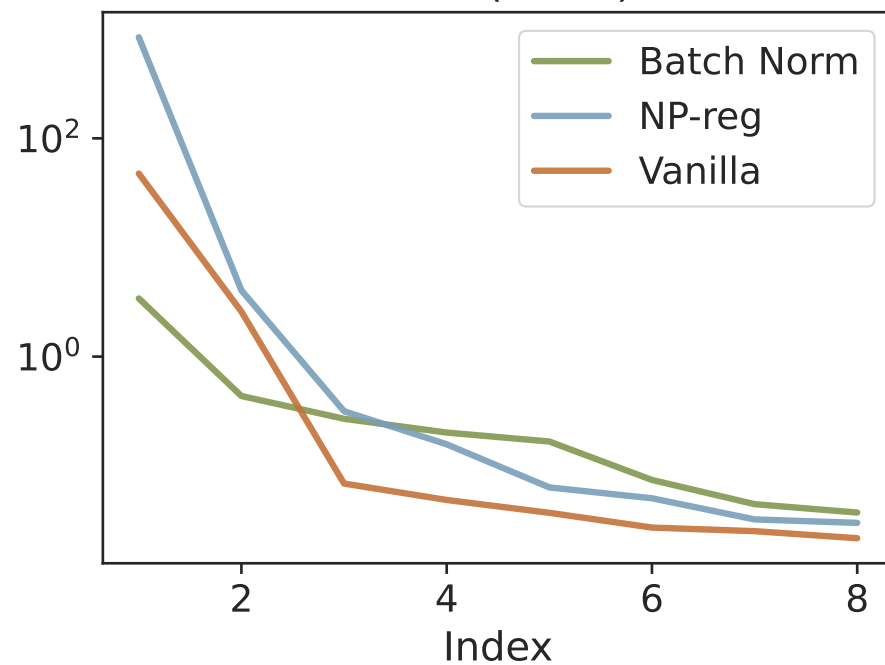
IMDb (small)
