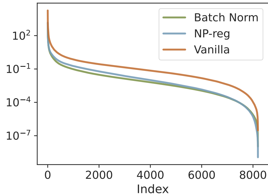
CIFAR-10
