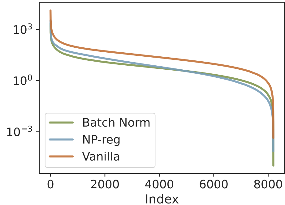
CIFAR-10
