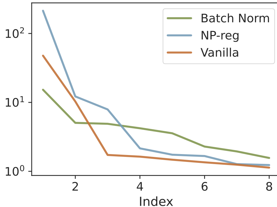
IMDb (small)
