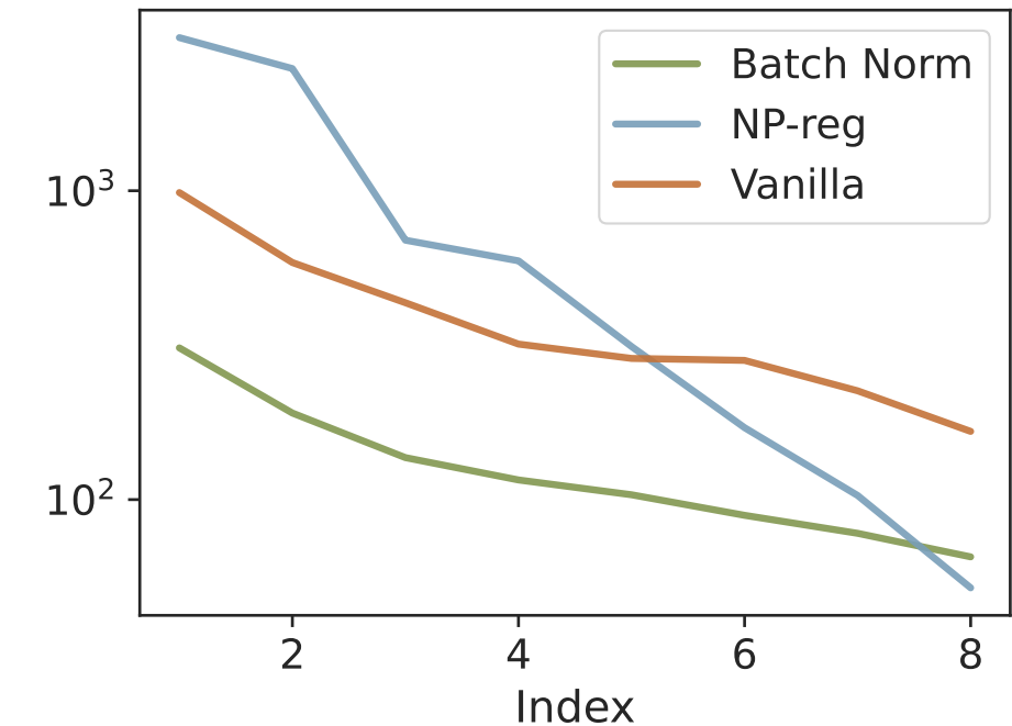
CIFAR-10 (small)
