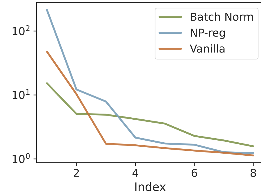
IMDb (small)
