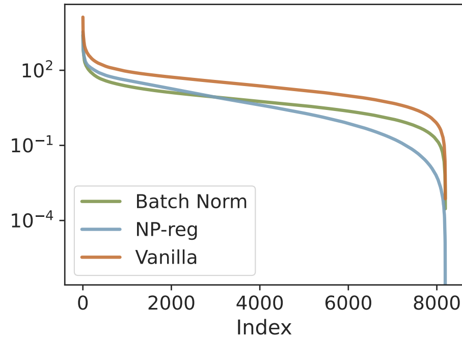
CIFAR-10
