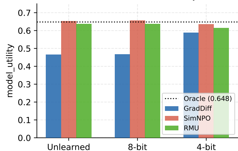
Quantization — model utility
