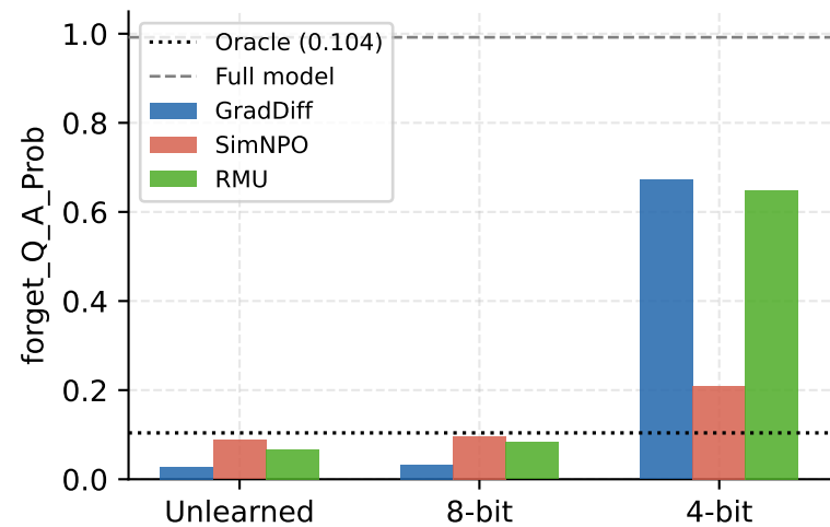
Quantization — knowledge recovery
