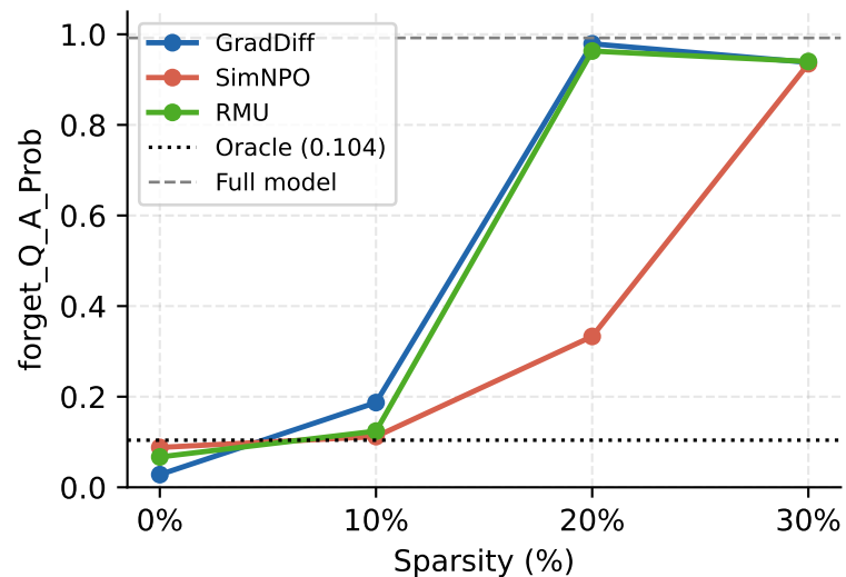
Pruning — knowledge recovery
