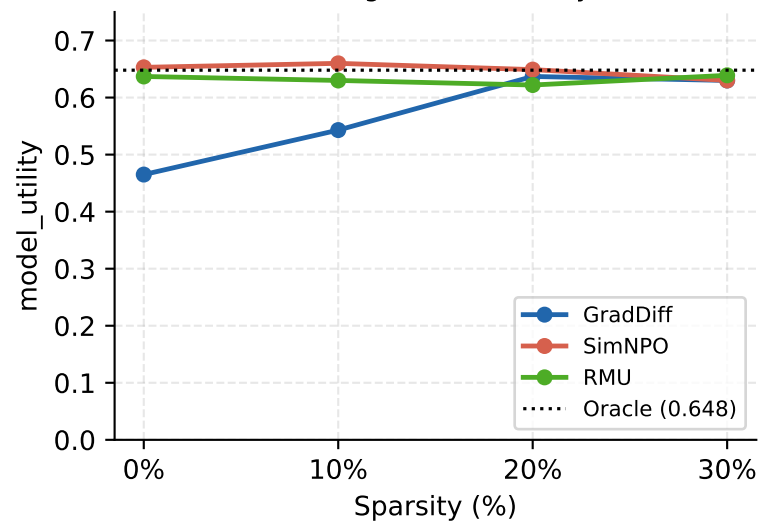
Pruning — model utility
