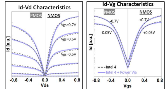
Fig. 5. Transistor Id-Vg and Id-Vd characteristics for both N/P MOS are matched between Intel 4 and Intel 4+PowerVia.
