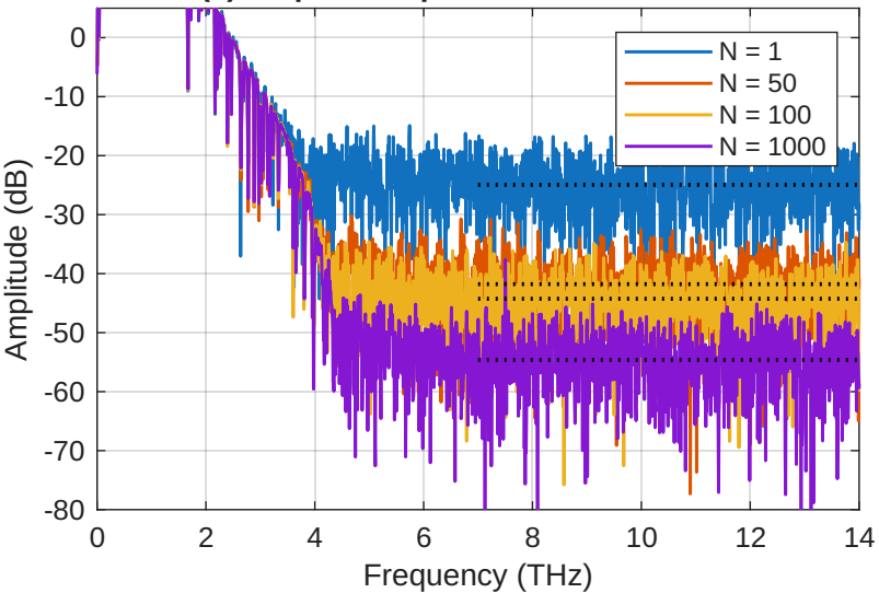
(a) Amplitude spectra and noise floors
