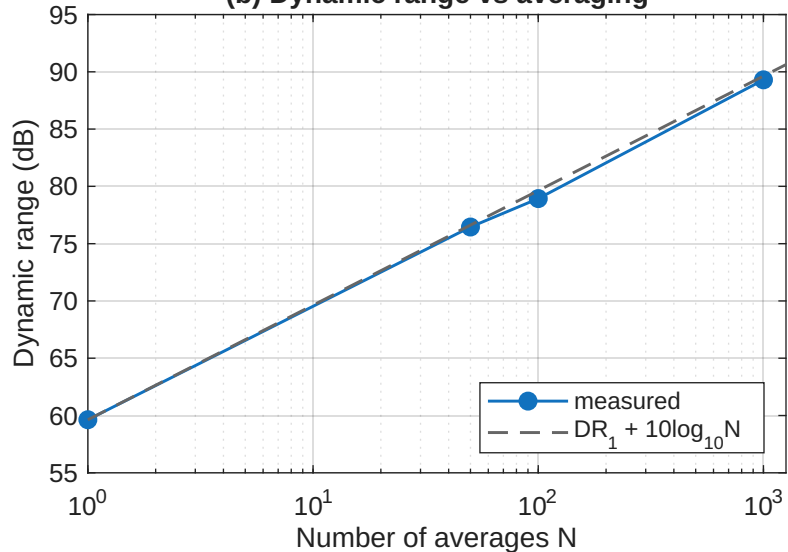
(b) Dynamic range vs averaging
