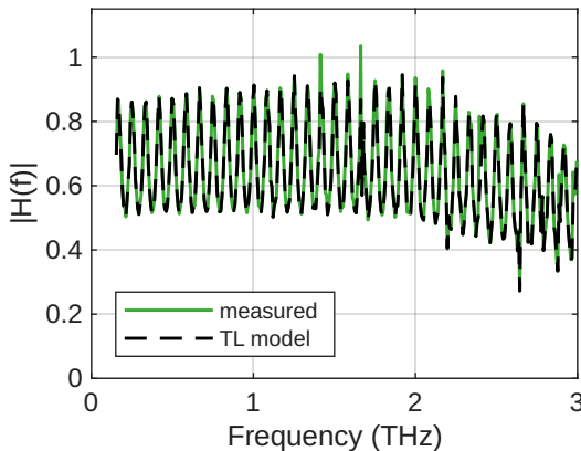
Slab 5: \epsilon_r = 11.66 , \tan\delta = 0.004
