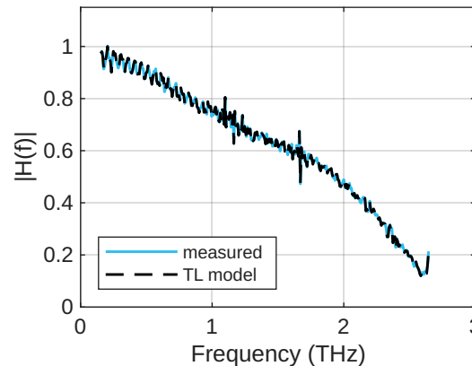
Slab 6: \epsilon_r = 2.05 , \tan\delta = 0.010
