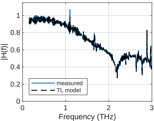
Slab 4: \epsilon_r = 11.72 , \tan\delta = 0.010
